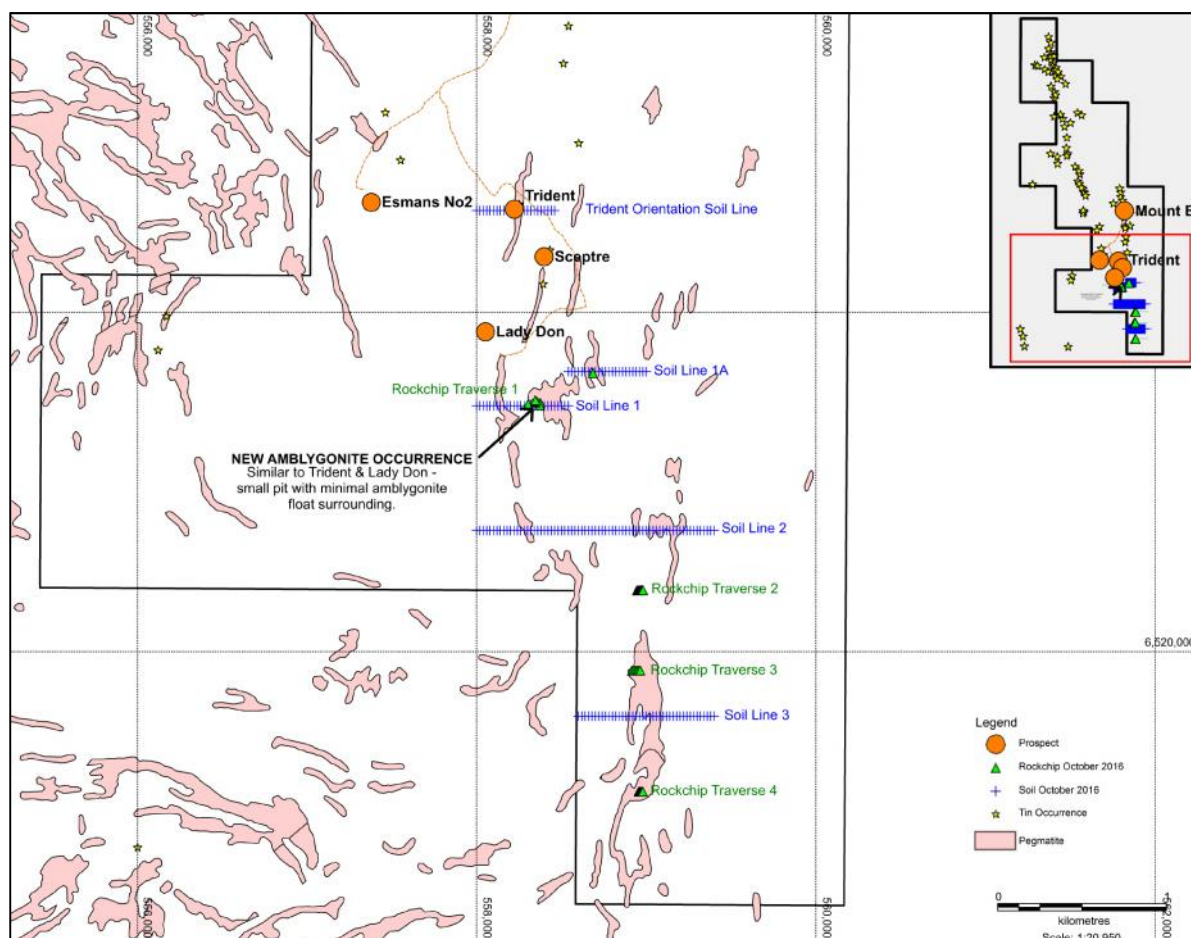
Figure 1. Plan of geochemical exploration completed over southern amblygonite target at the Euriowie project.
