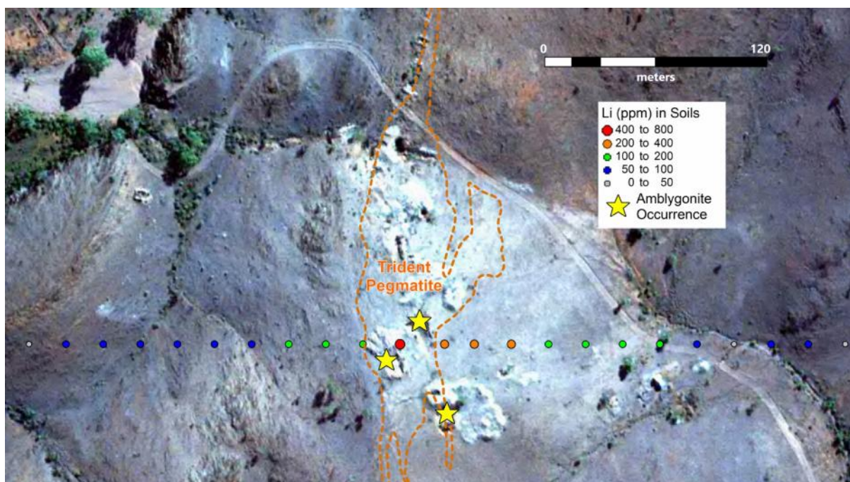
Figure 3. Orientation soil line over Trident pegmatite showing anomalous (>100 ppm Li) Li over a 200 m wide zone, with an 80 m wide core zone (>200 ppm Li).
