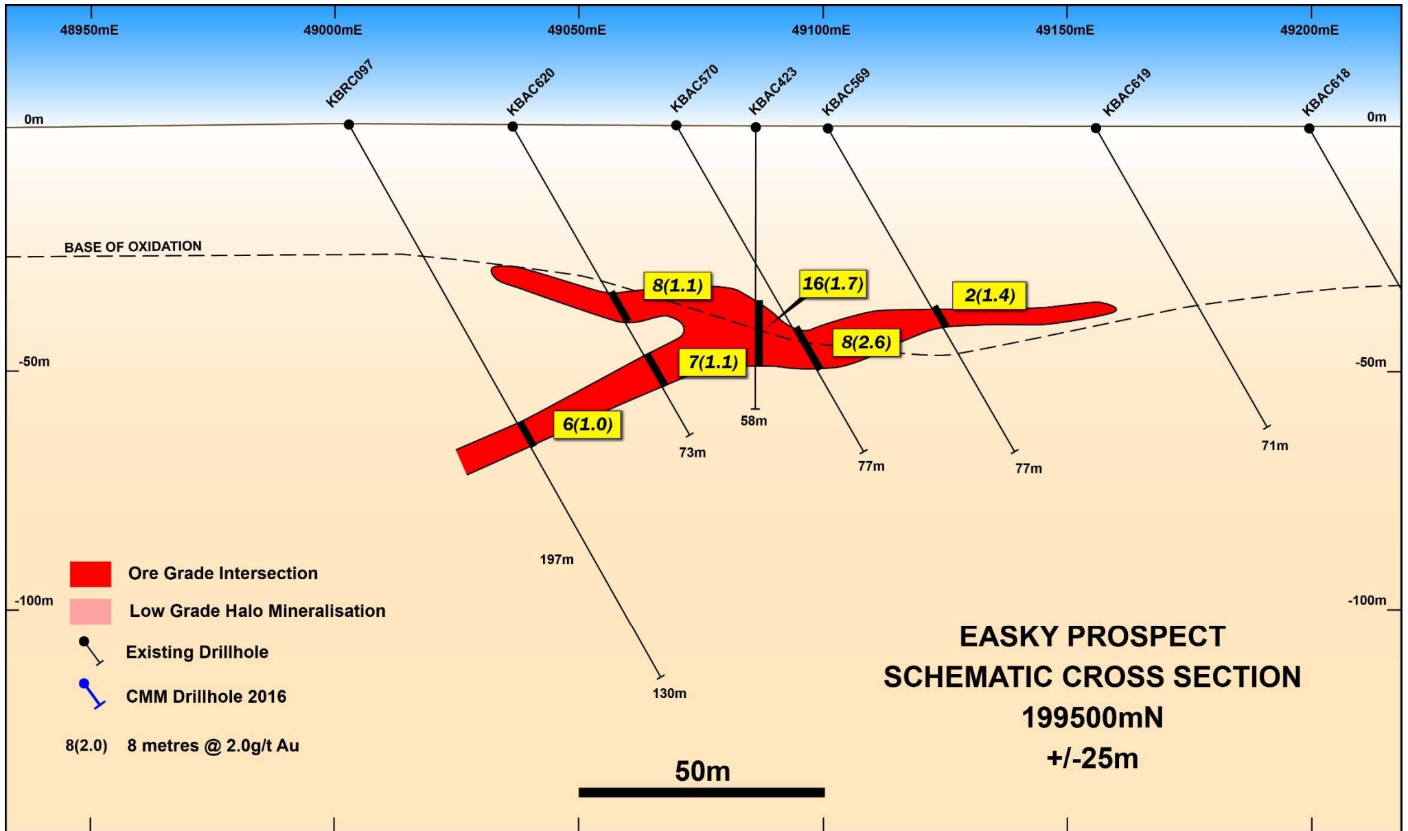
Figure 3: Easky Cross Section 199500mN
