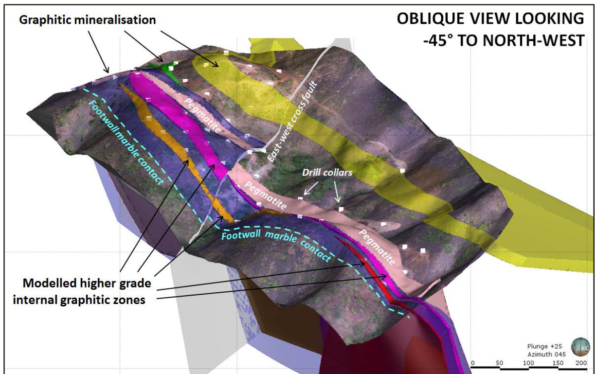
Figure 3. View of Cascade geology showing zones of graphitic mineralisation.
