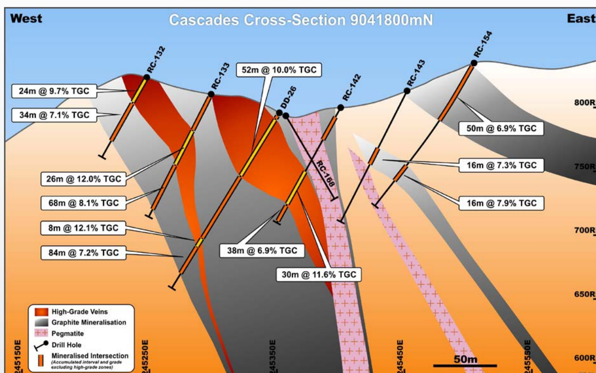
Figure 2. Cascades cross section at 9041800N showing graphite mineralisation on ridge structure.
