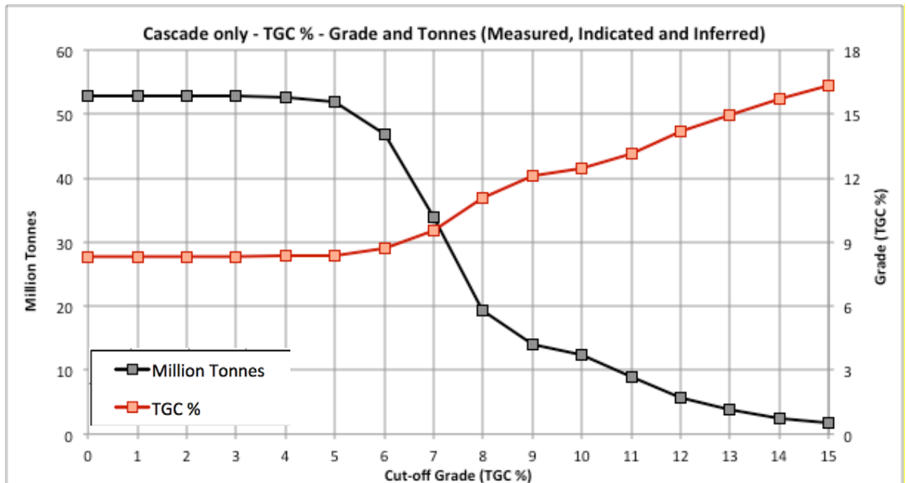
Graph 2. Global Mahenge TGC% grade-tonnage curve
