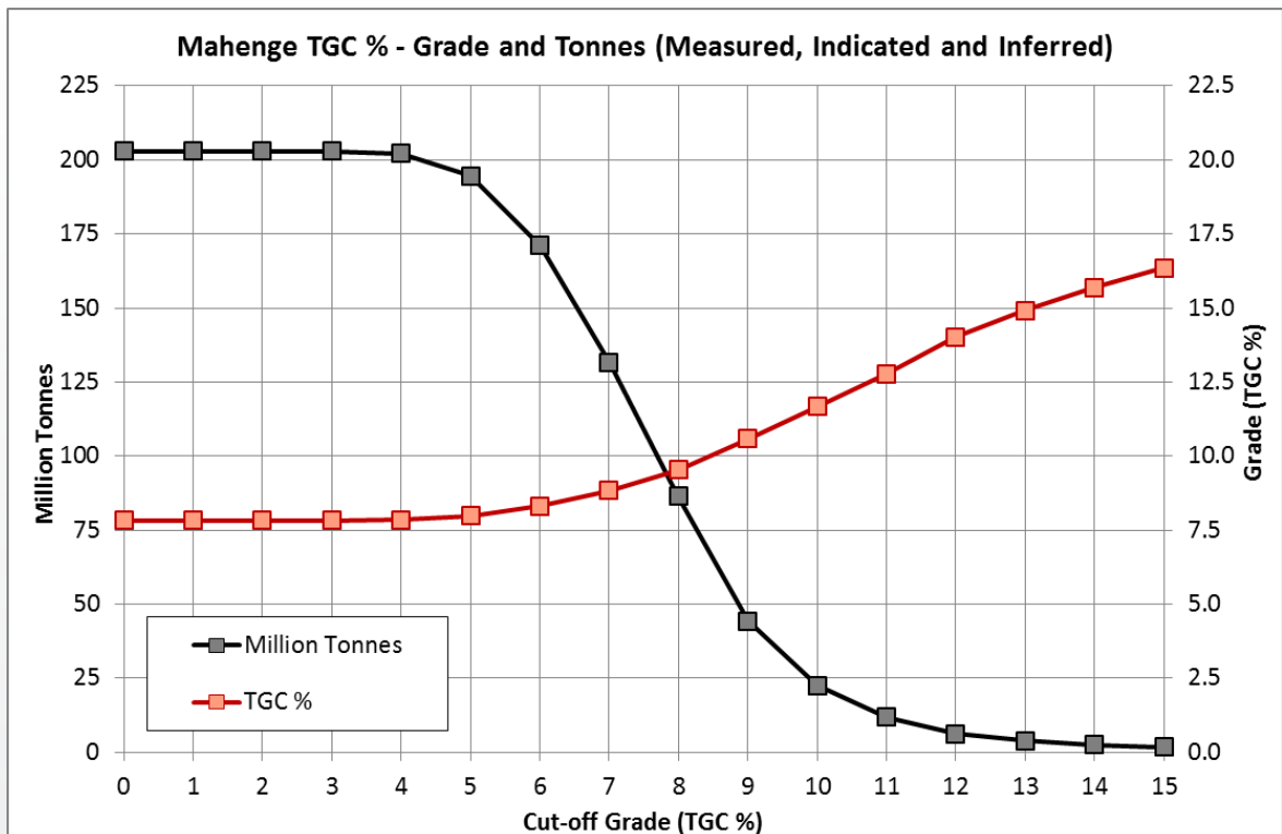
Graph 1. Global Mahenge TGC% grade-tonnage curve
