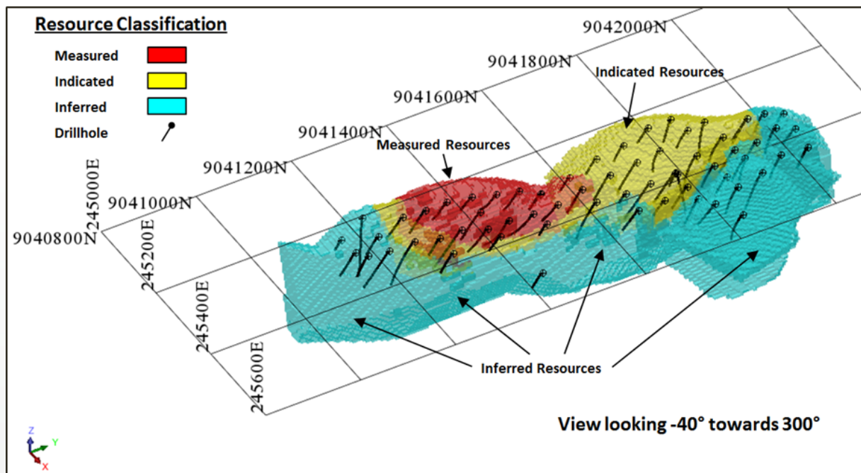
Figure 4. View of Cascade block model showing zones of Measured, Indicated and Inferred Resources.
