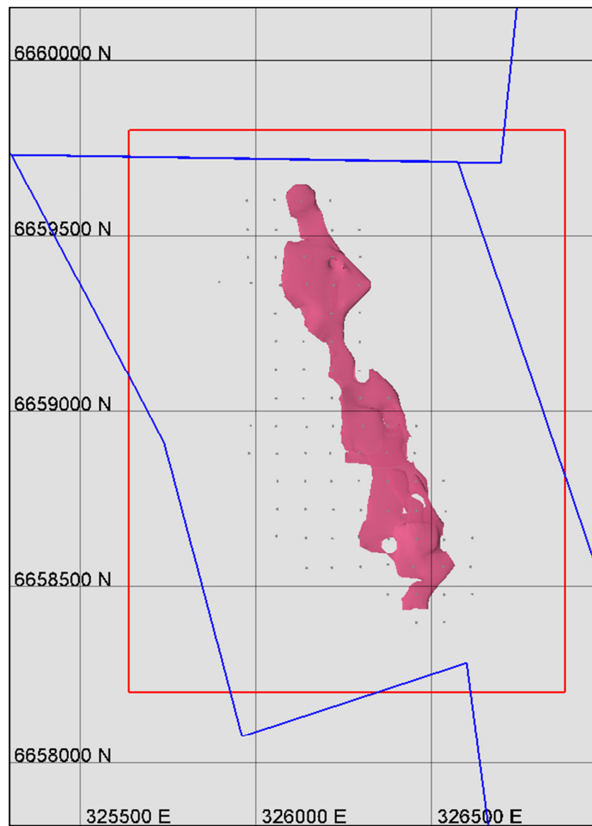
Figure 7: - Scotia - trimmed grade shell based on 0.08% Co cutoff
