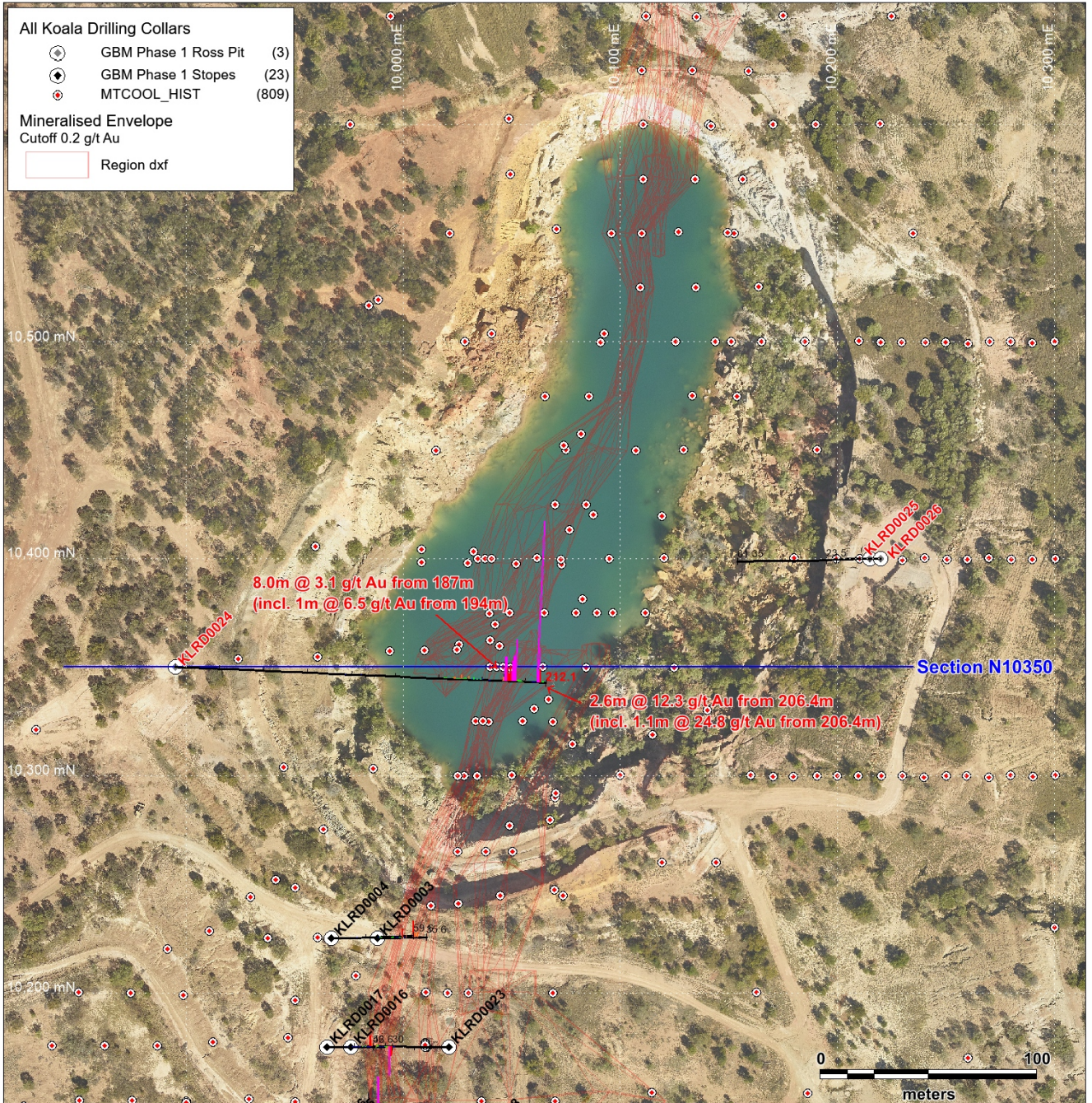
Figure 1: Koala North Pit drill hole plan showing down hole intersections. Underlying high resolution image is from 2016 LIDAR survey. Grid is a local non-earth grid.
