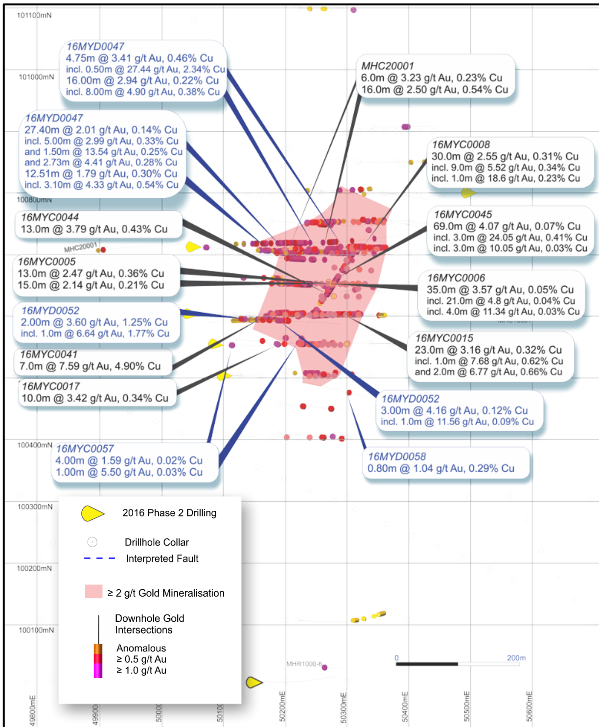
Figure 2: Minyari Deposit plan view showing drill hole locations and plan projection of approximate boundary of \geq 2.0 g/t gold mineralisation with selected 2016 drill hole intercepts. Note: Labelled 2016 Phase 2 drill hole intercepts in blue.
