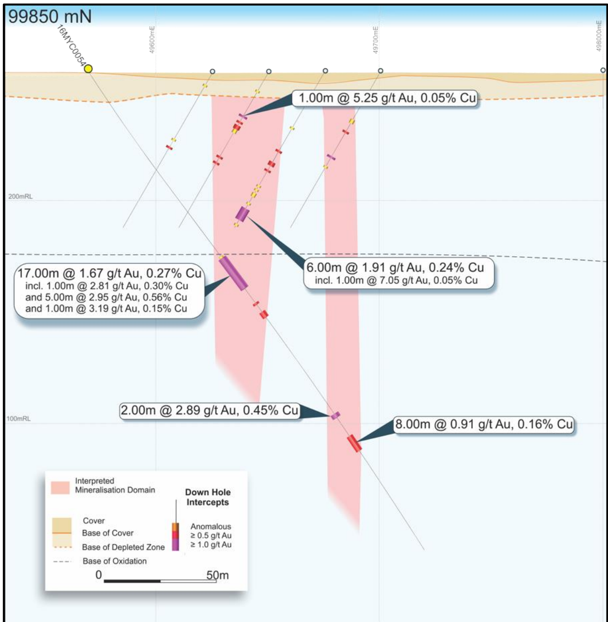
Figure 6: WACA Deposit 99850 North interpreted (schematic) cross-section (looking north) showing drill holes, including 2016 Phase 2 RC drill hole, with gold grade bars and interpreted gold-copper mineralisation domains (100m elevation grid).
