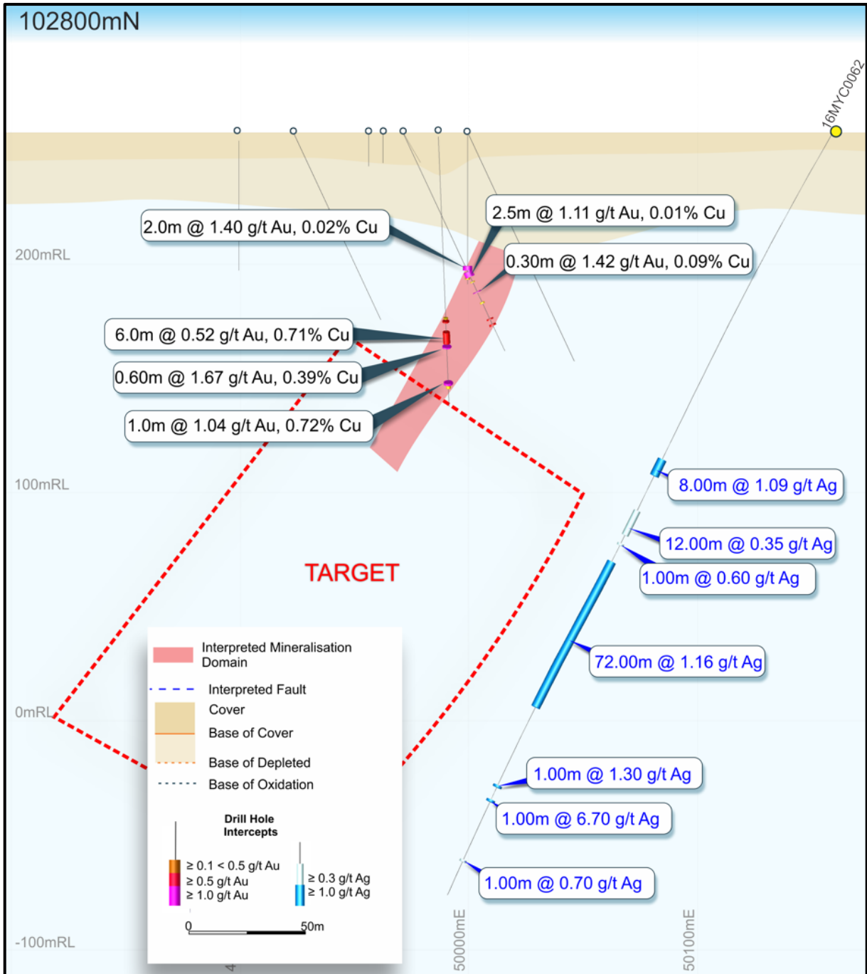
Figure 8: Jude's East area 102800 North interpreted (schematic) cross-section (looking north) showing drill holes, including 2016 Phase 2 RC drill hole, with gold grade bars and interpreted gold-copper mineralisation domain, extensive "path-finder" silver intercepts and target area (100m elevation grid).
