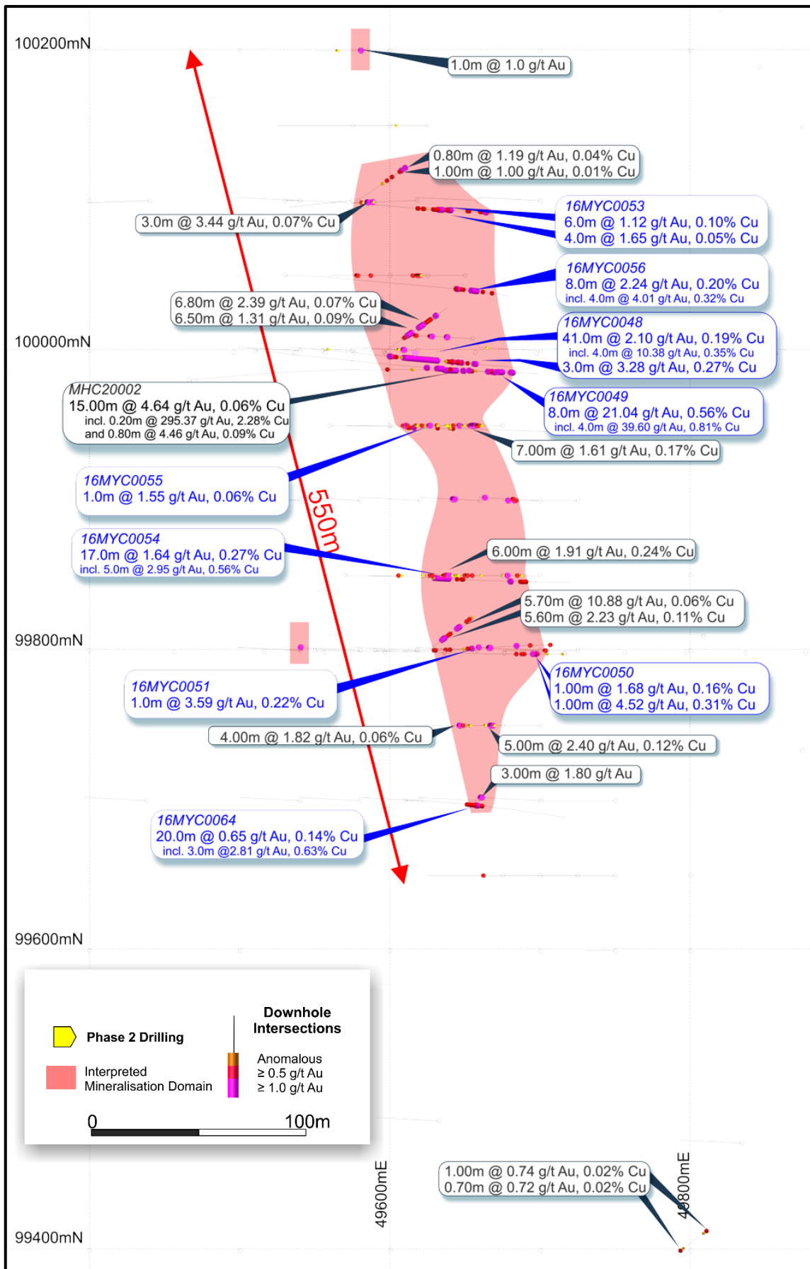
Figure 5: WACA Deposit plan view showing drill hole locations and generalized plan projection of approximate boundary encapsulating 1.0 g/t gold mineralisation. Note: Labeled 2016 Phase 2 RC drill hole intercepts in blue.
