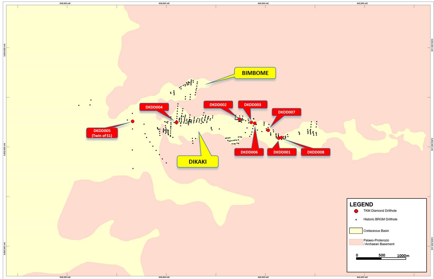
Figure 3: Drillhole collar plan of the Dikaki channel showing the historic drilling and the spread of the current drilling being undertaken by Trek Metals.
