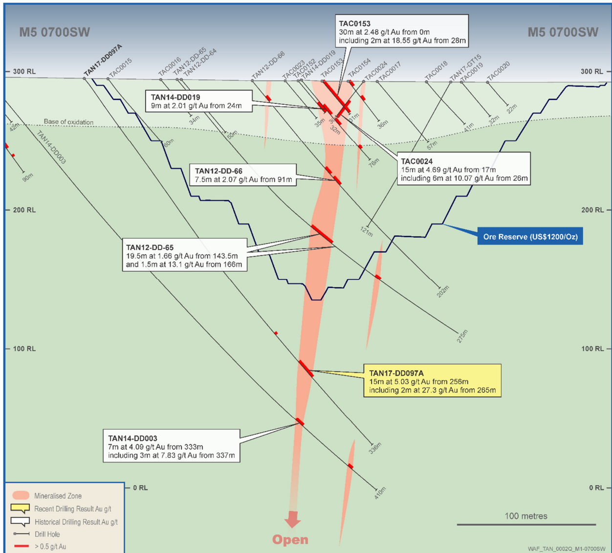
Figure 4: M5 Section SW700
