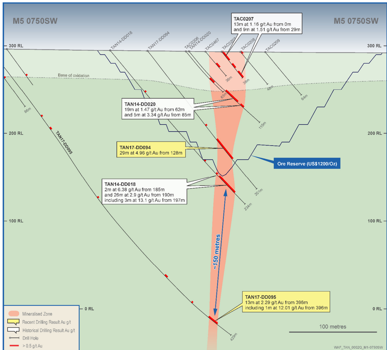
Figure 5: M5 Section SW750
