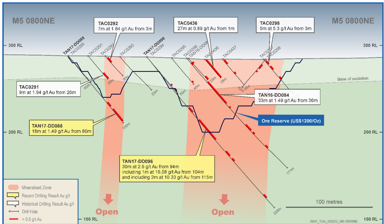
Figure 6: M5 Section NE800 (Northern Zone)
