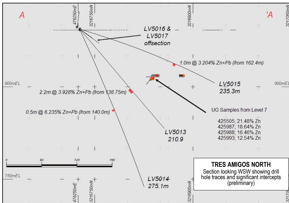
Figure 5. Cross section through Tres Amigos North looking WSW showing drill traces and significant preliminary assay results to date. Note location of UG samples showed in Figure 3 plan.
