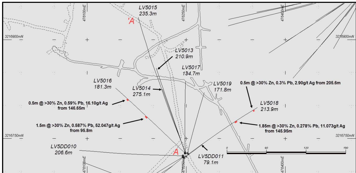
Figure 4. Drill traces and preliminary assay results from drillholes targeting Tres Amigos North and the face sampling grades shown in Figure 3. Cross section A-A' is shown in Figure 5.
