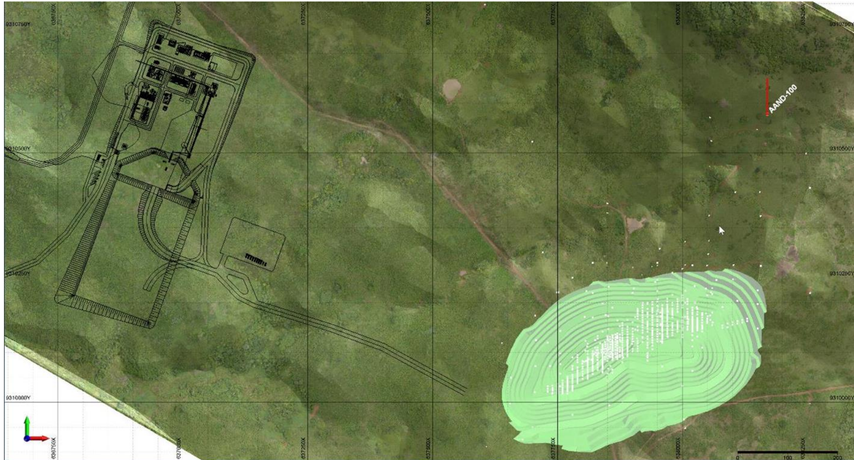
Figure 5: Surface Plan Showing Location of AAND-100 in Proximity to the Antas Pit and Mine Infrastructure
