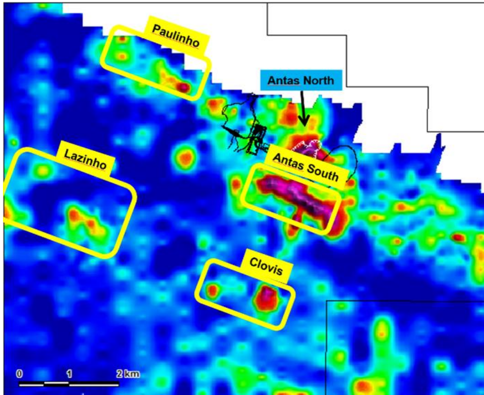
Figure 4: Near Mine Targets Shown Over Copper in Soil Anomalism (coloured hot to cold)
