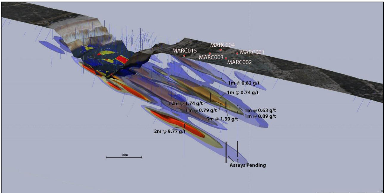
Figure 2: Lady Ada oblique section looking North, showing the drill targets against the extent of the current mineral resource model and the exploration drilling results.
