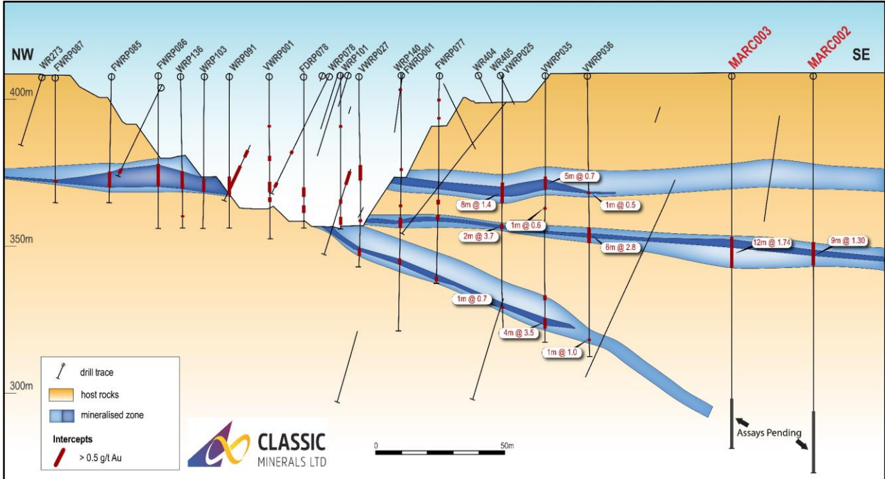
Figure 1: Lady Ada cross section looking north east showing CLZ drill holes
