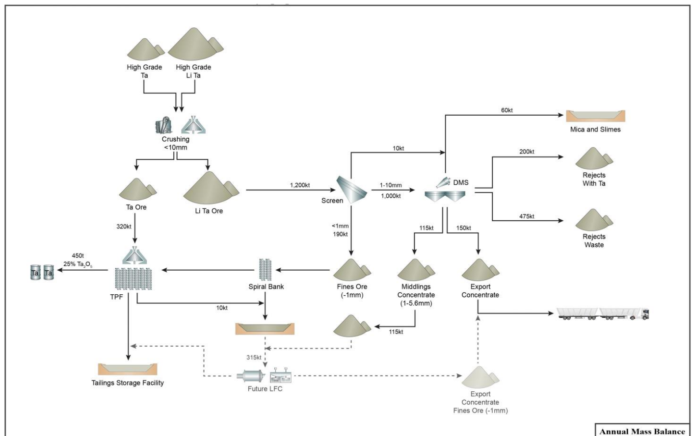
Figure 5: Simplified Process Flow and Mass Balance Diagram
