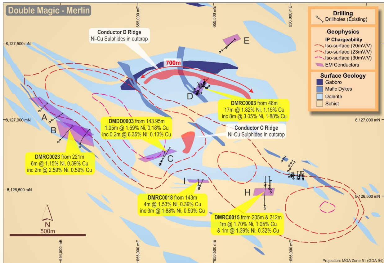
Figure 2 – Simplified geology, geophysical responses, and previously reported 2015 drillhole intersections, Merlin Prospect
