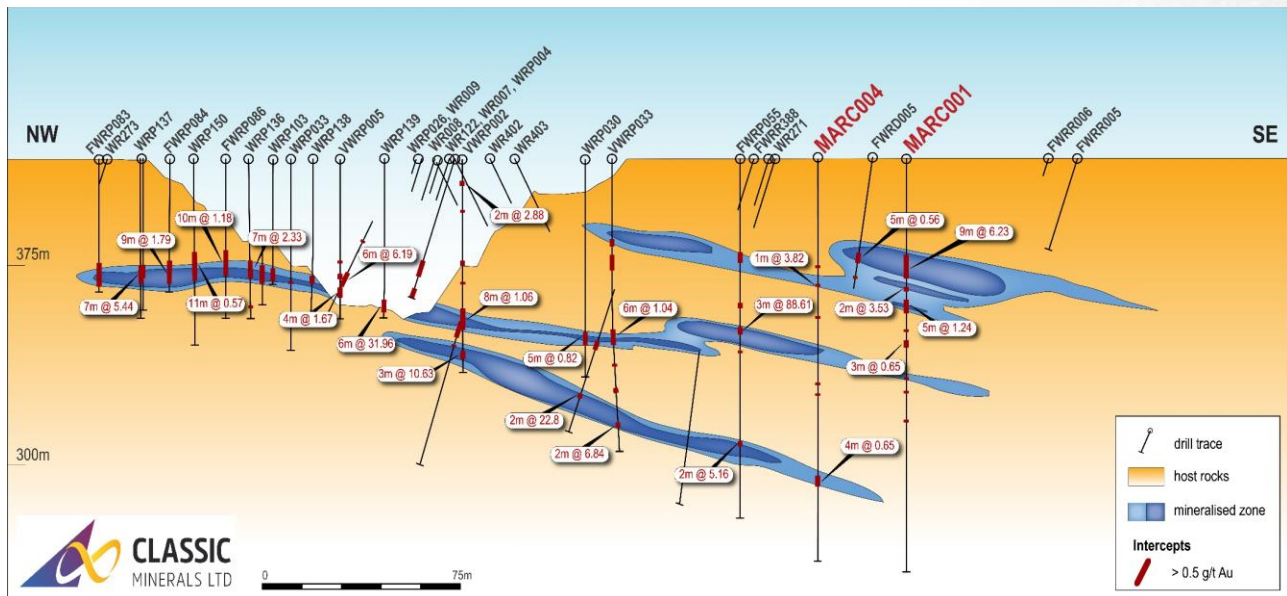
Figure 1: Lady Ada cross section looking north east showing CLZ drill holes MARC001 and MARC004
