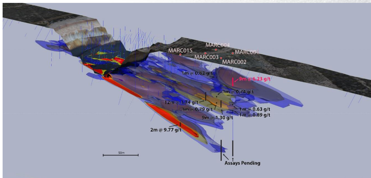
Figure 2: Lady Ada oblique section looking North, showing the implicit mineralisation model and the exploration drilling results.
