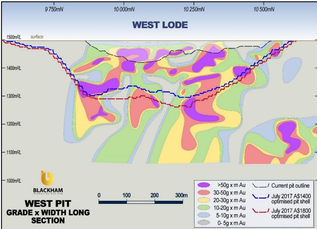
Figure 3. Long section through the deepest section of the West pit showing that the A$1,400/oz optimised pit shell is only slightly smaller than the A$1,800/oz pit shell
