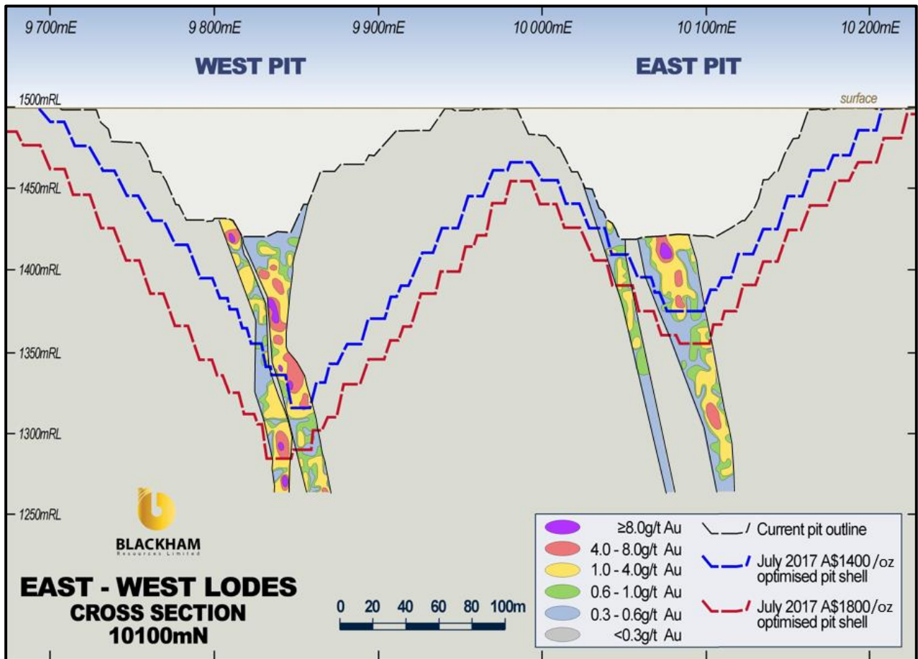
Figure 4. Cross section A-A' through the East-West pit looking north comparing the July A$1,800/oz and A$1,400/oz optimised pit shells
