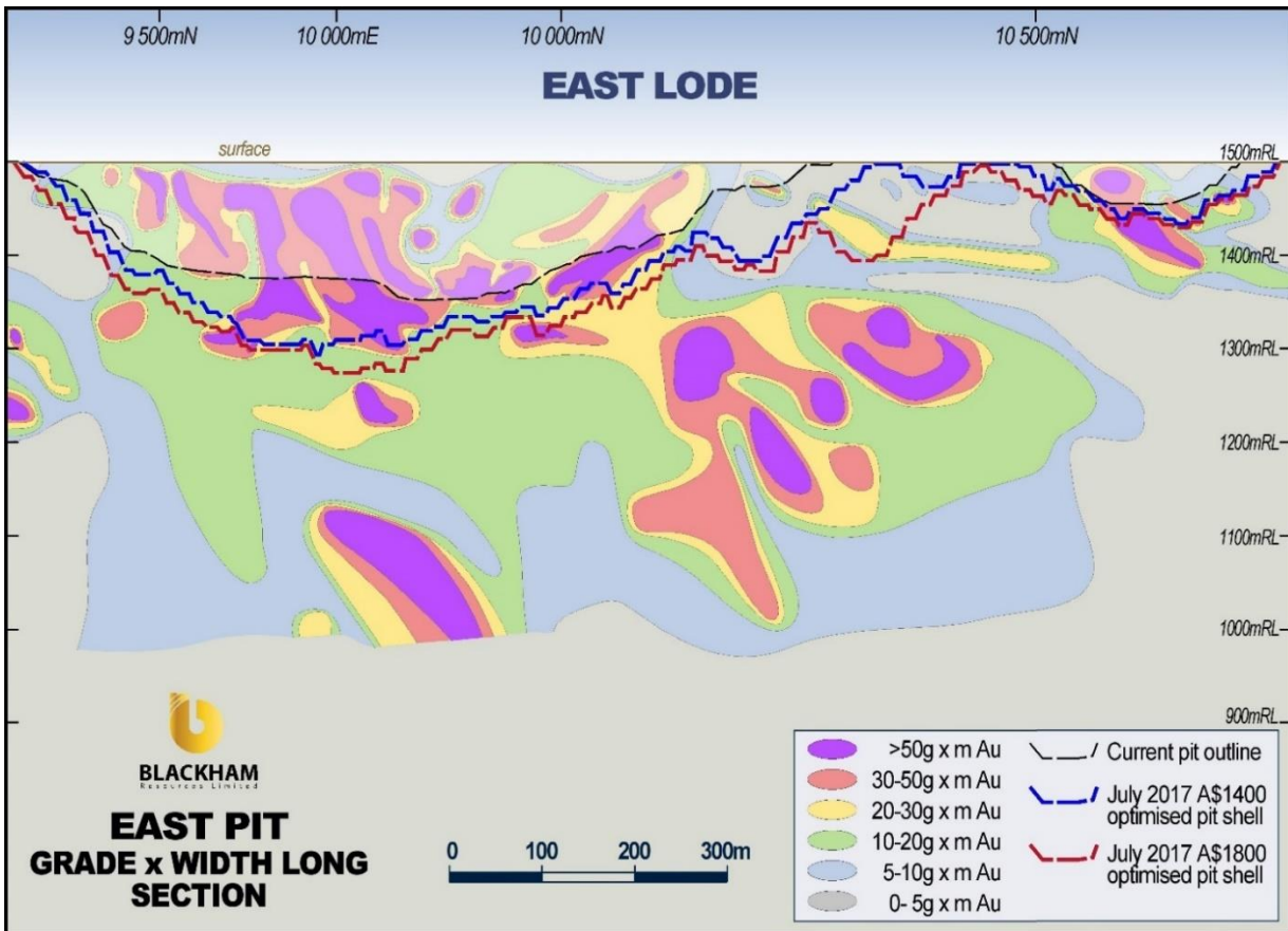
Figure 2. Long section through the deepest section of the East pit showing that the A$1,400/oz optimised pit shell is only slightly smaller than the A$1,800/oz pit shell
