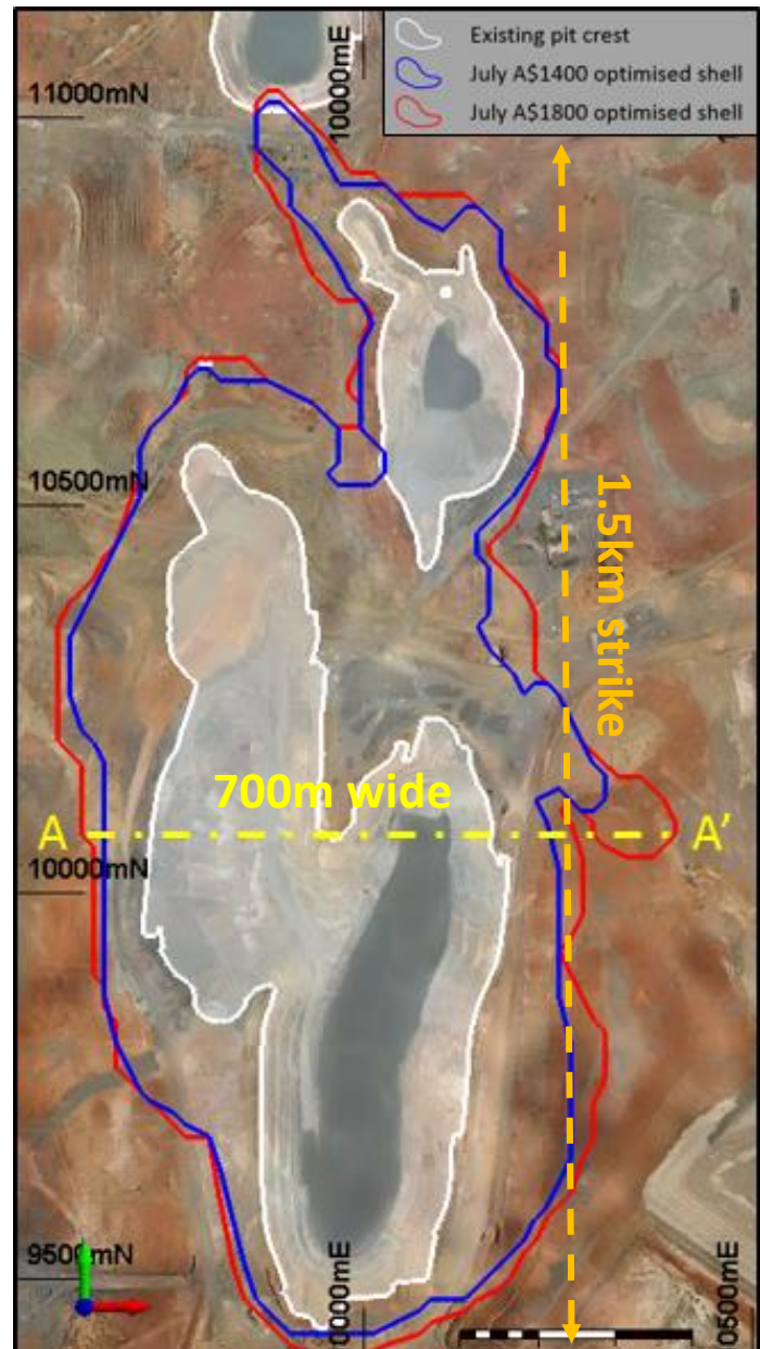
Figure 1. Comparison between the A$1400/oz and A$1,800/oz optimised pit shells shows that there is little difference between the footprints of the potential pits. Consequently it is likely that the Resource to Reserve conversion is likely to be high. Location of cross section A-A' (Figure 4) shown
