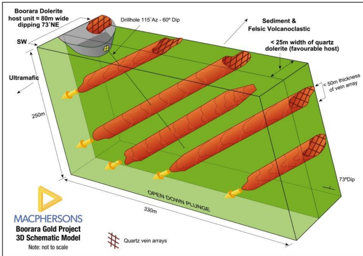
Figure 2: Boorara geological model schematic showing quartz vein arrays and current drill azimuth
