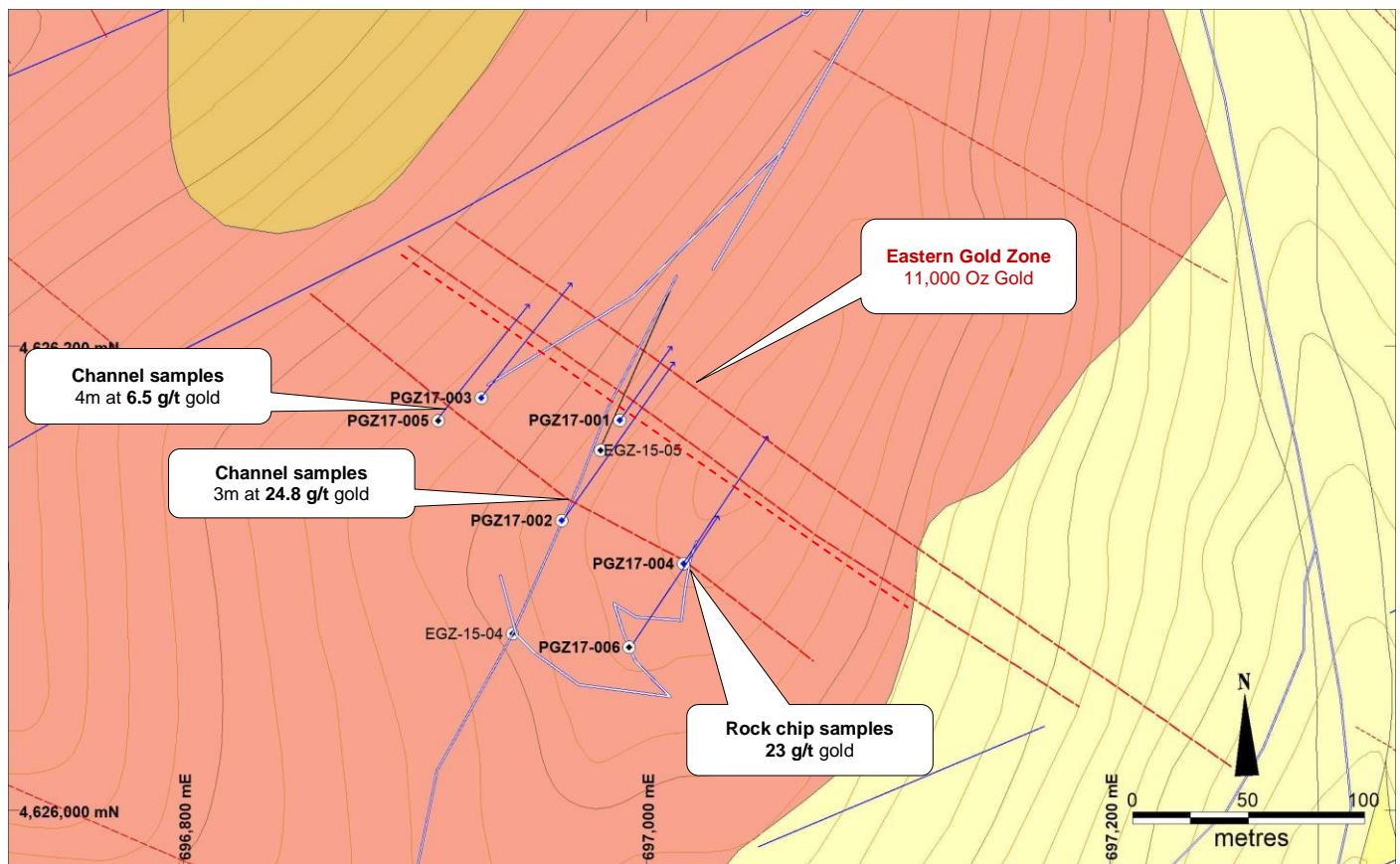
Figure 1: Plan of drilling at the Eastern Gold Zone showing channel sampling results and structural interpretation. See figure 3 for the location of the Eastern Gold Zone relative to the other mineralised zones at Aucu.
