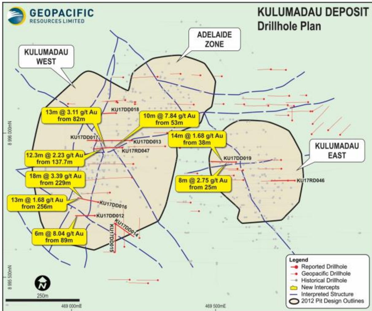
Figure 2: Drill hole location plan for Kulumadau
