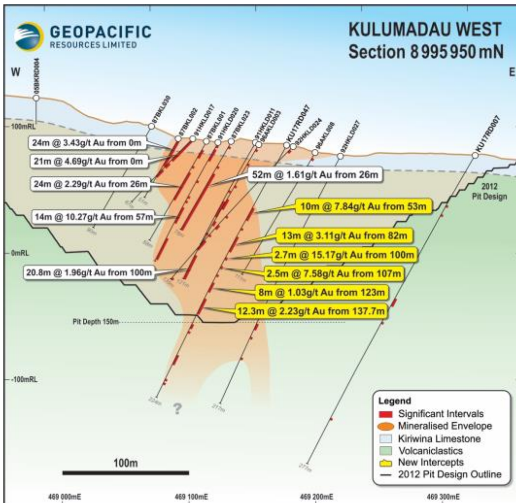
Figure : Cross section of Kulumadau West showing mineralised intersections in KU17RD047
