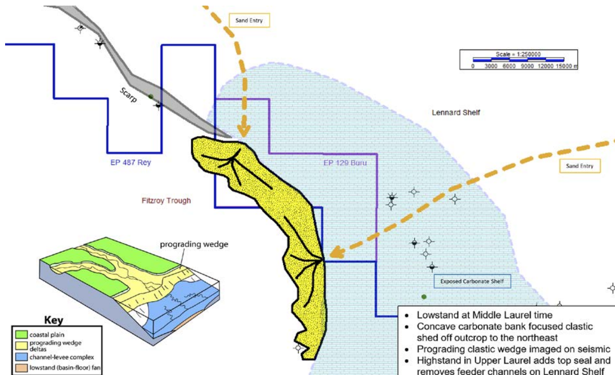
Figure 2: The Butler Prospect shown in depositional form in the North-East corner of EP 487.
