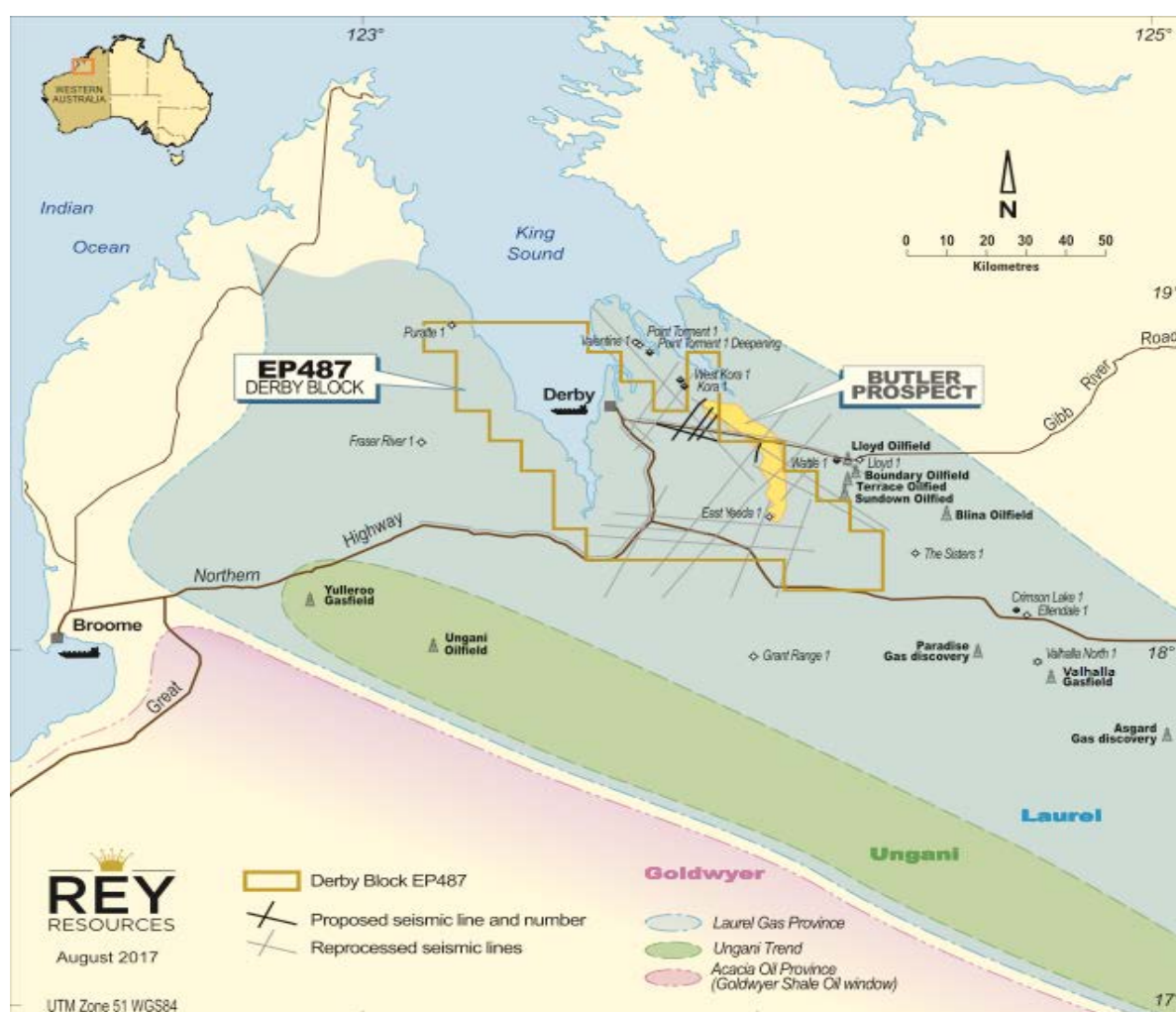
Figure 1: Location Plan of New 2D Seismic
