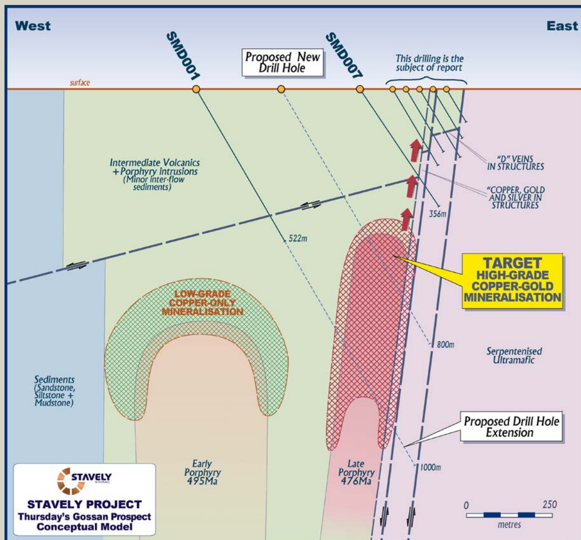
Figure 4. Stavely Minerals' conceptual model of two-phase porphyry intrusion with the second-phase porphyry driving the copper-gold-silver mineralisation with some leakage to surface along structures.
