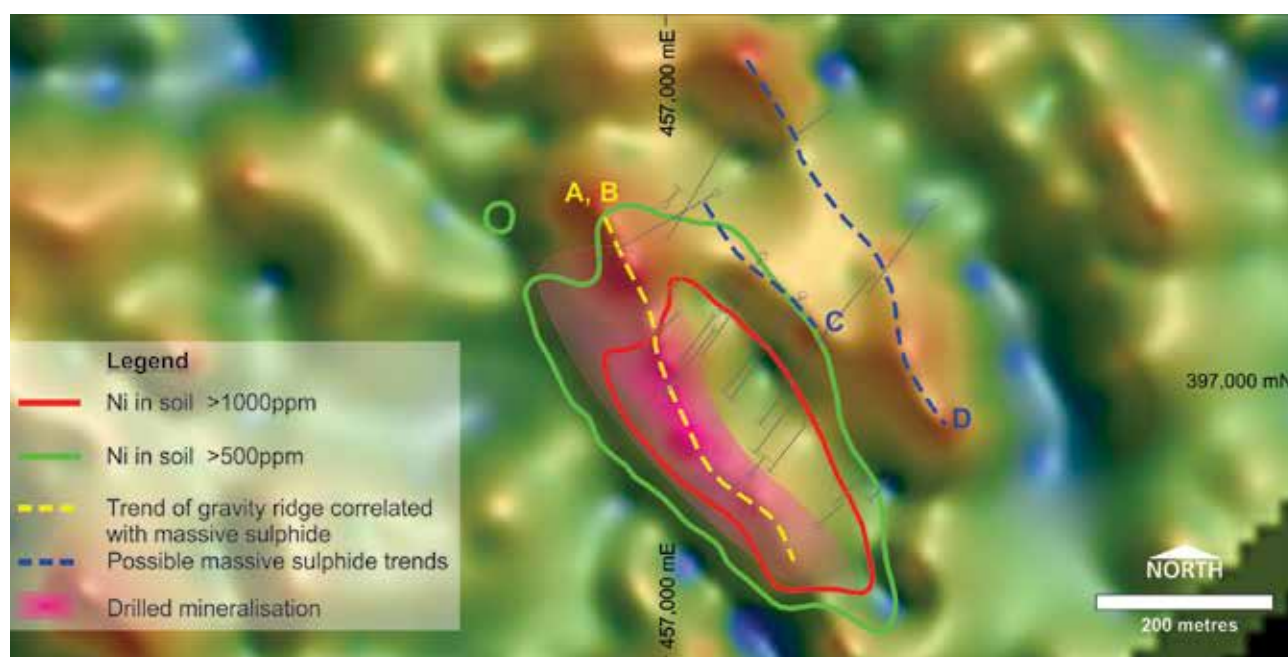
Figure 10: Showing 1VD of residual Bouguer gravity with known and interpreted massive sulphide trends from DHTEM and drilling. Note all trends are open down plunge and outcrop to the south east.
