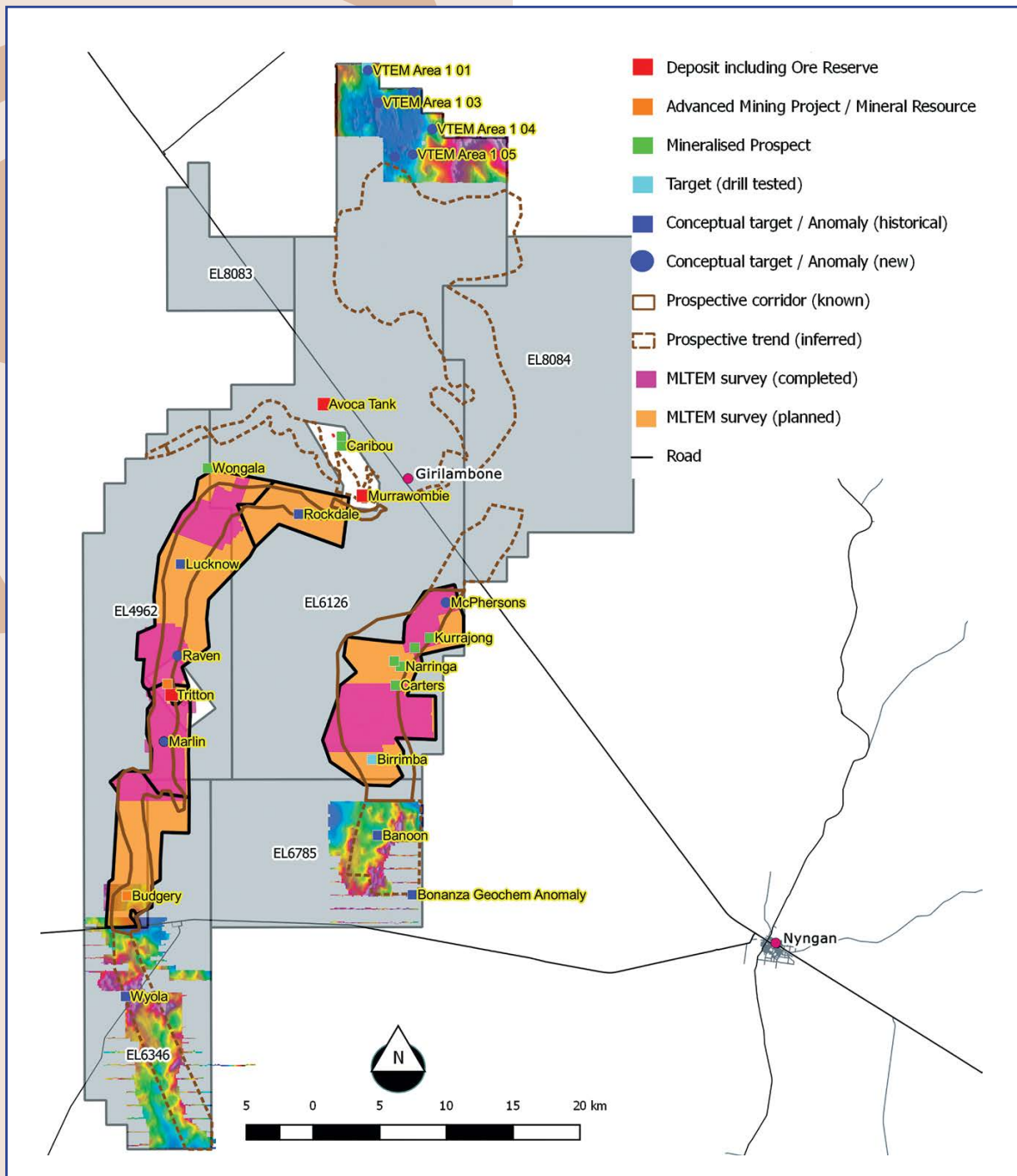
Tritton region showing Aeris Tritton tenement package and prospective corridors for copper mineralised systems. The planned MLTEM geophysical survey coverage is highlighted by shaded orange regions and completed survey areas by shaded magenta regions.
