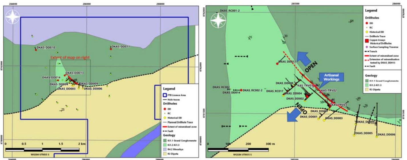
Figure 2: Prospect-scale map of Kasangasi showing extent of mineralised zone and area of artisanal workings.
