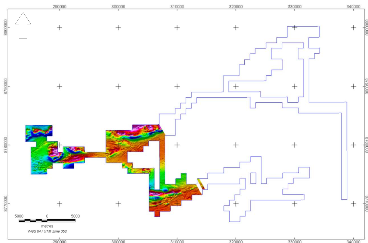
Figure 7: Progress of the airborne magnetic survey.
