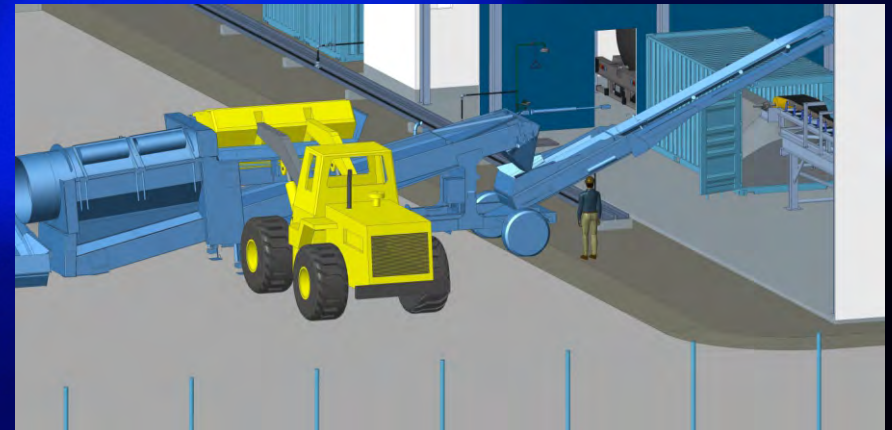
PROPOSED MECKERING KAOLIN SCREENING AND LOADING FACILITY LAYOUT
