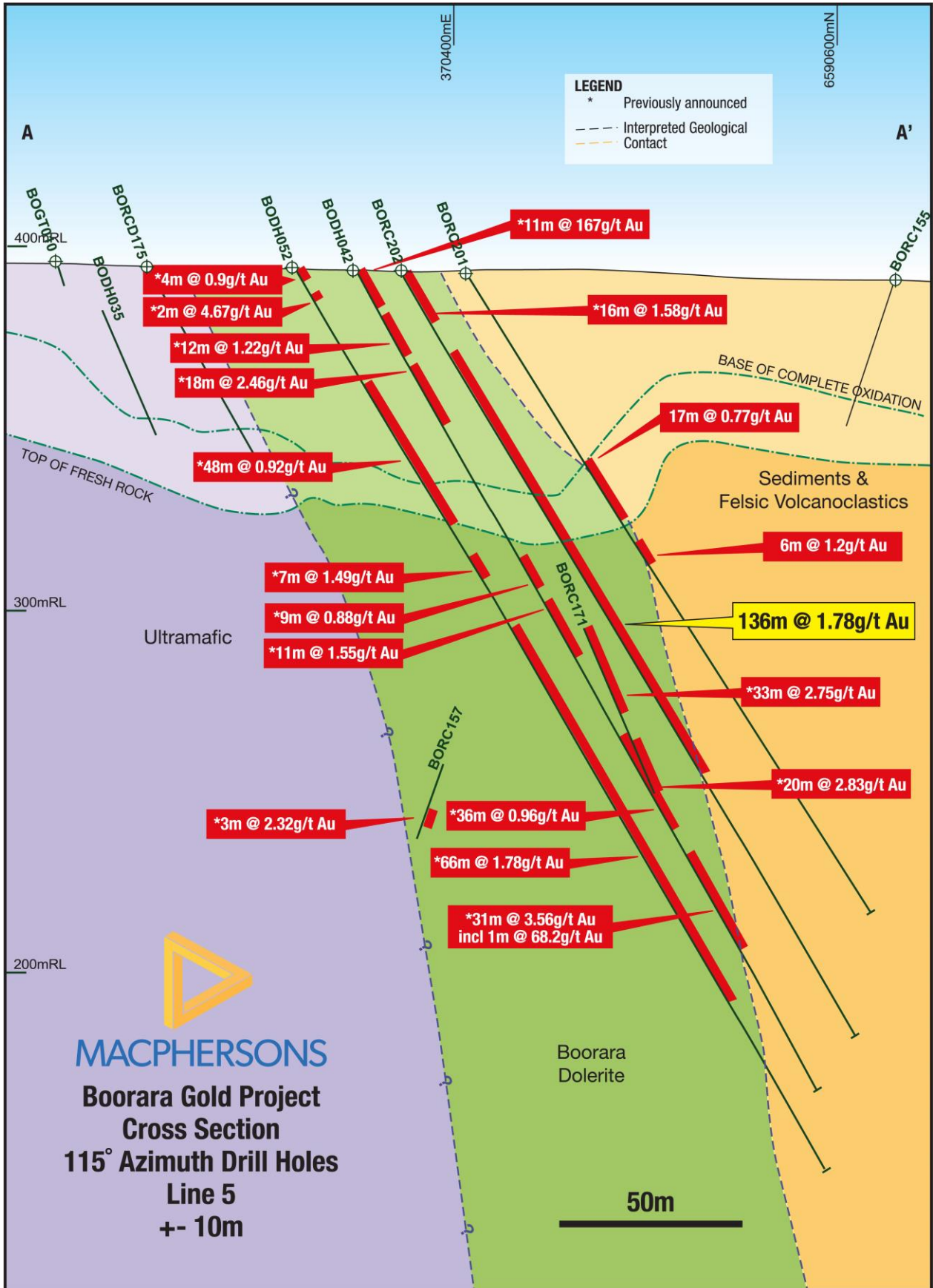
Figure 4: Cross section view of BORC 201 & 202 with interpreted geology.
