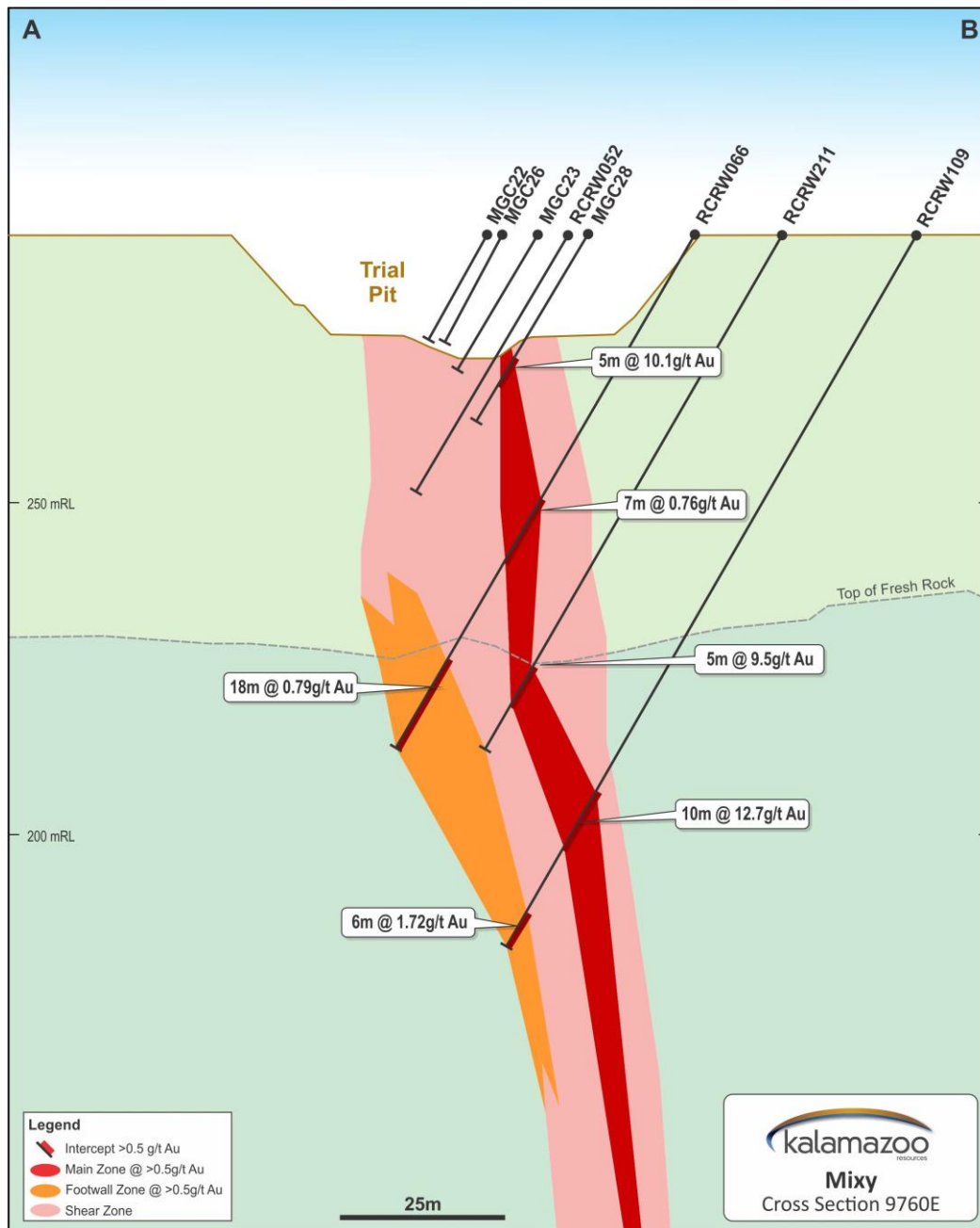
Figure 6: Mixy Cross Section A-B looking east within the resource outline (Intersections are down hole lengths of >0.5 g/t Au, and include a maximum of 2m at <0.5 g/t Au)
