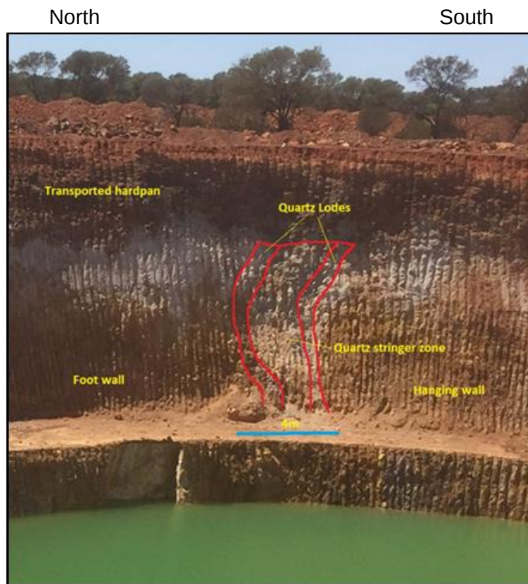
Figure 4. Photo of Eastern Wall of Mixy Trial pit and positions of the Main Zone gold veins and inter-vein alteration and quartz stringer zone. Blue bar is ~4m.
