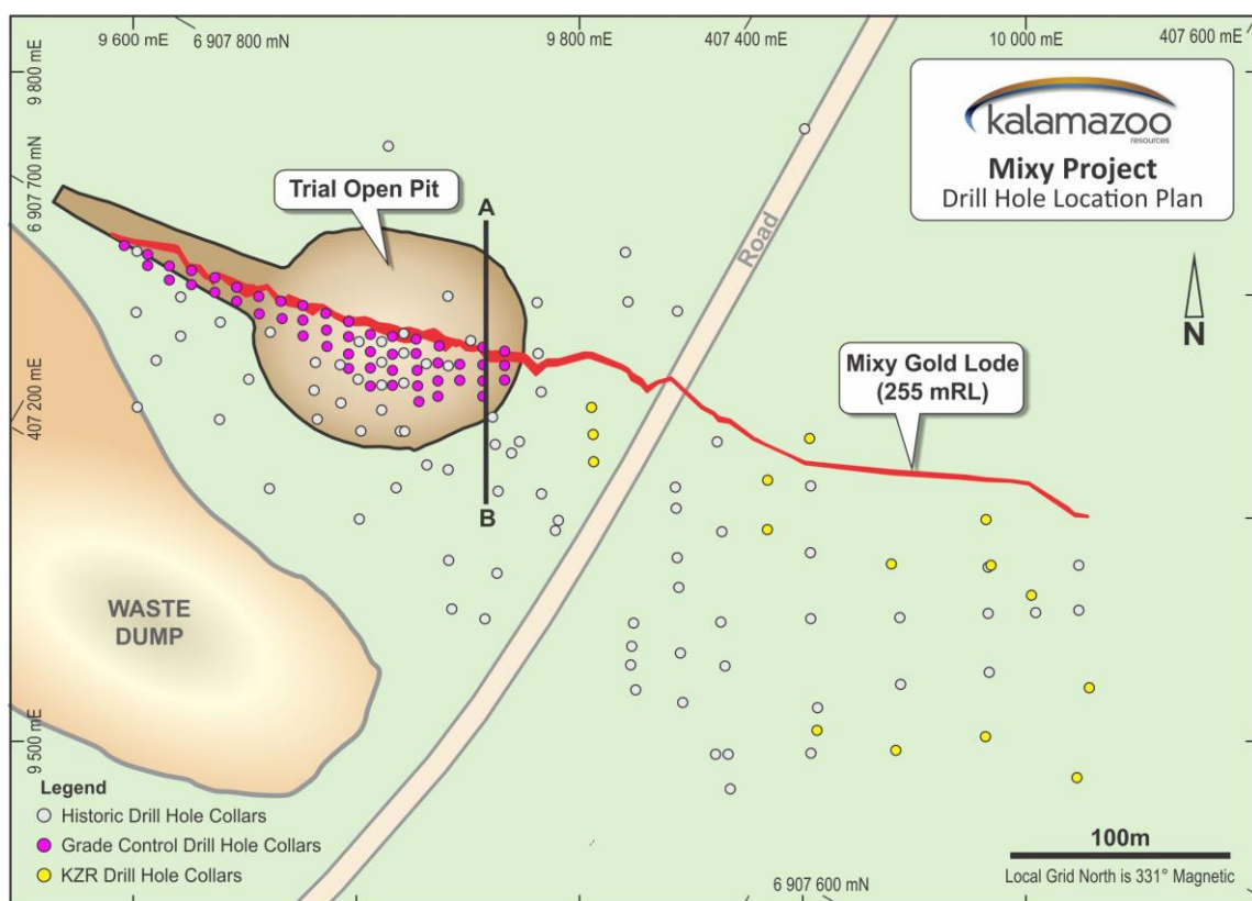
Figure 2: Location plan of Mixy trial pit, drill holes and cross section (orientated to local grid North)
