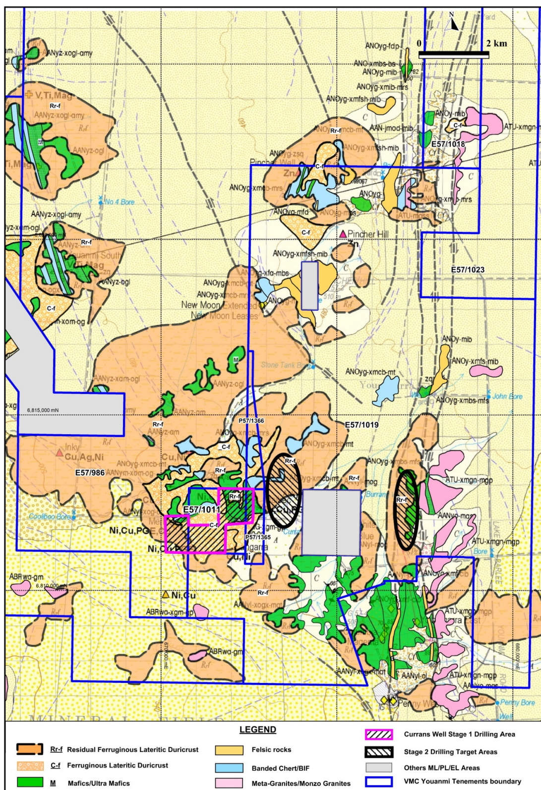
Figure 1. Location of Stage 1 Drilling and Stage 2 Drilling Target areas at Currans Well Co-Cu-Ni Project shown on GSWA 100k Geology
