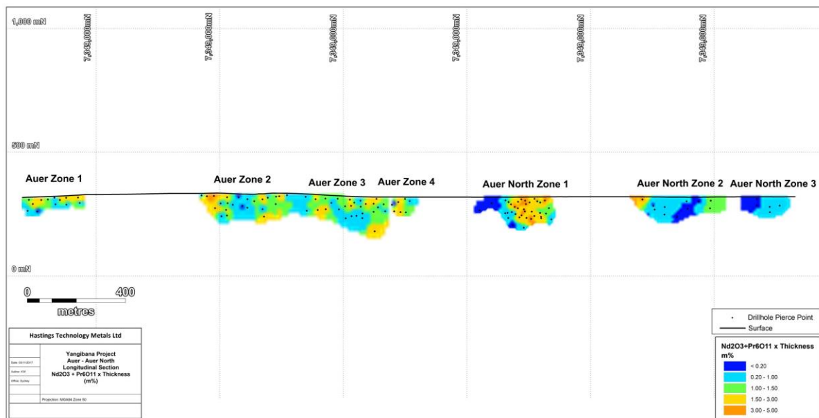
Figure 3 – Yangibana Project – Auer and Auer North m%Nd 2 O 3 +Pr 6 O 11 accumulations
