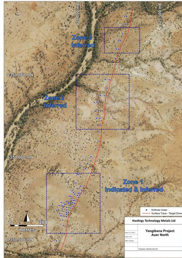
Figure 2 – Auer North drillhole locations
