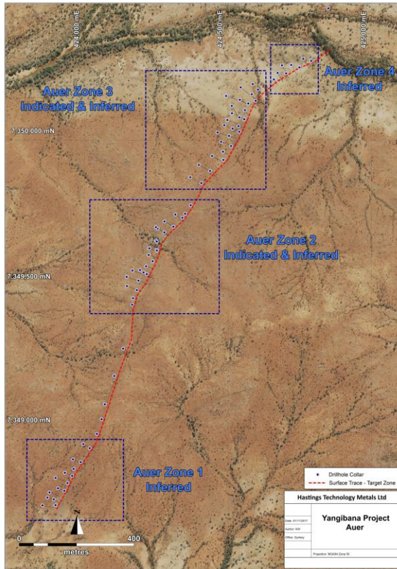
Figure 1 – Yangibana Project – Auer drillhole locations
