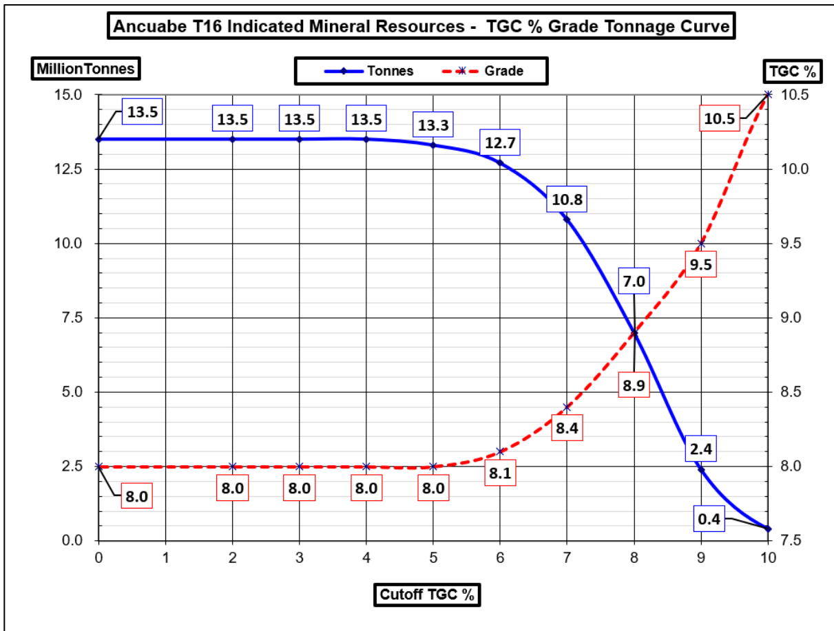
Figure 20: Grade Tonnage curve for Indicated Mineral Resources at T16
