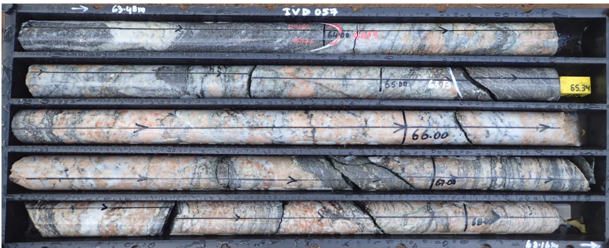
Figure 7: Pegmatitic pink feldspar layers and veins in the footwall rocks of IVD059
