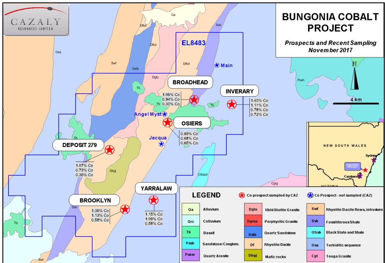
Figure 1. Geology, key prospects & recent sampling - Bungonia Cobalt Project
