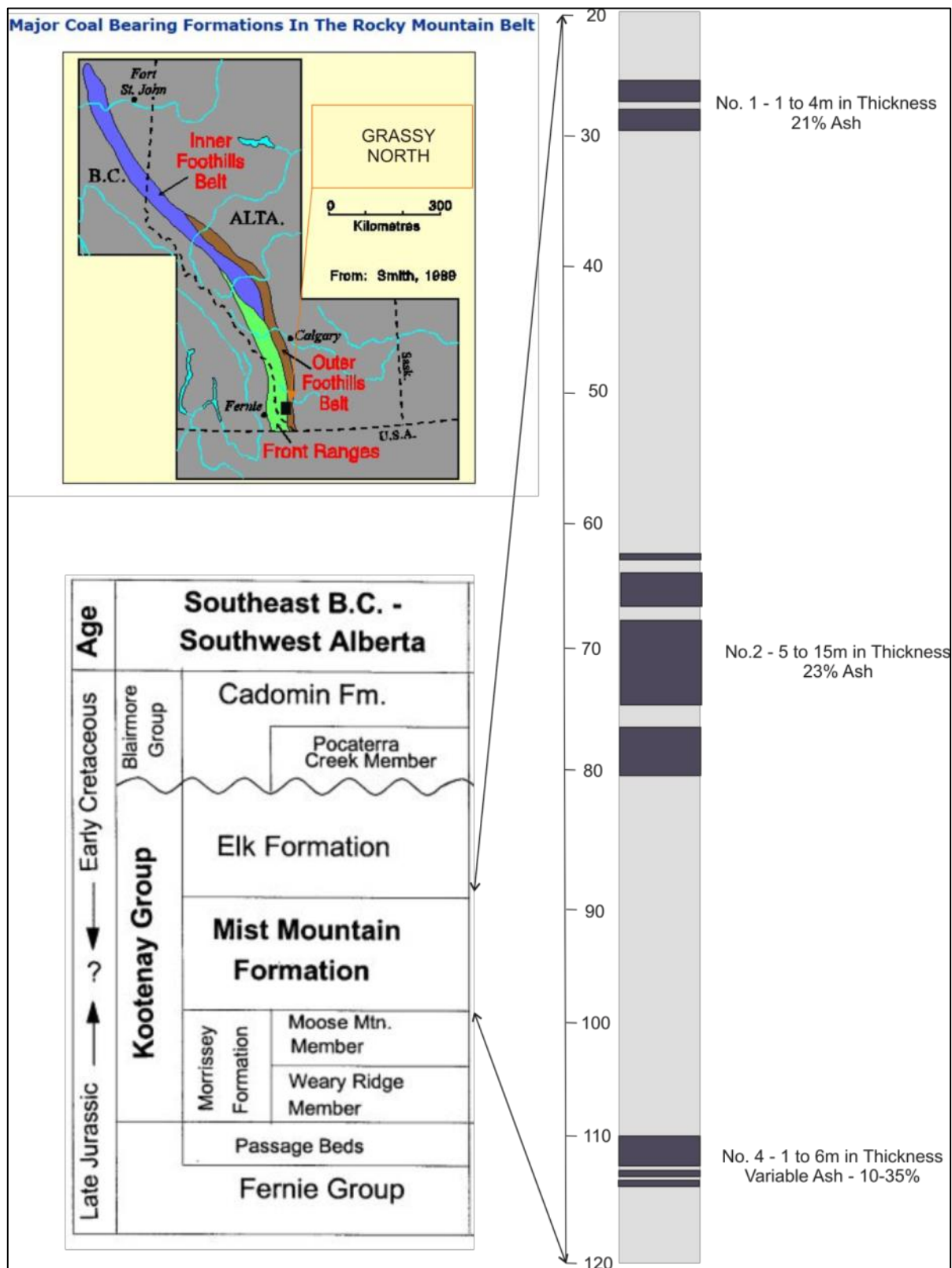
Figure 5 – Elan South Stratigraphy (ash% contents averages only)
