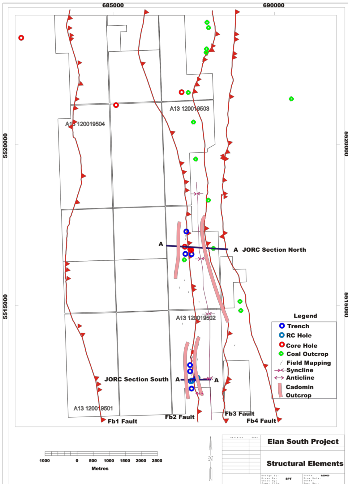
Figure 6 – Structure and Cross Section Locations
