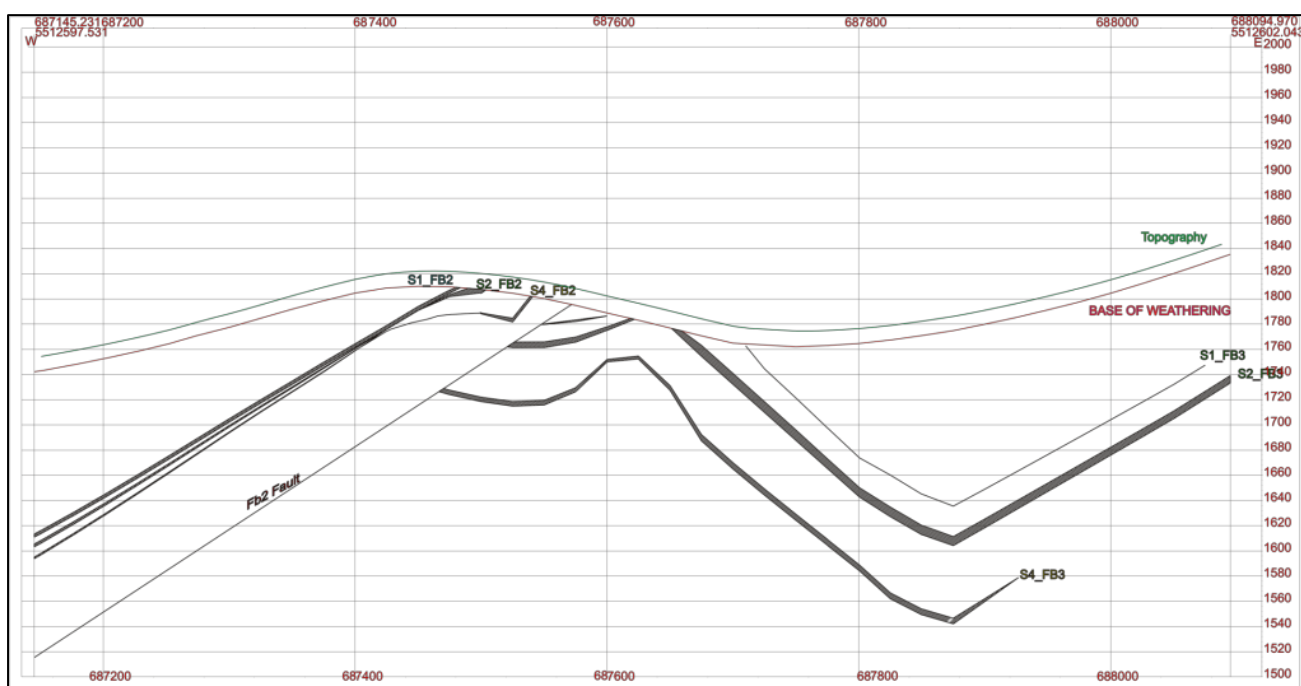
Figure 8 – Generic Cross Section – Southern Domain
