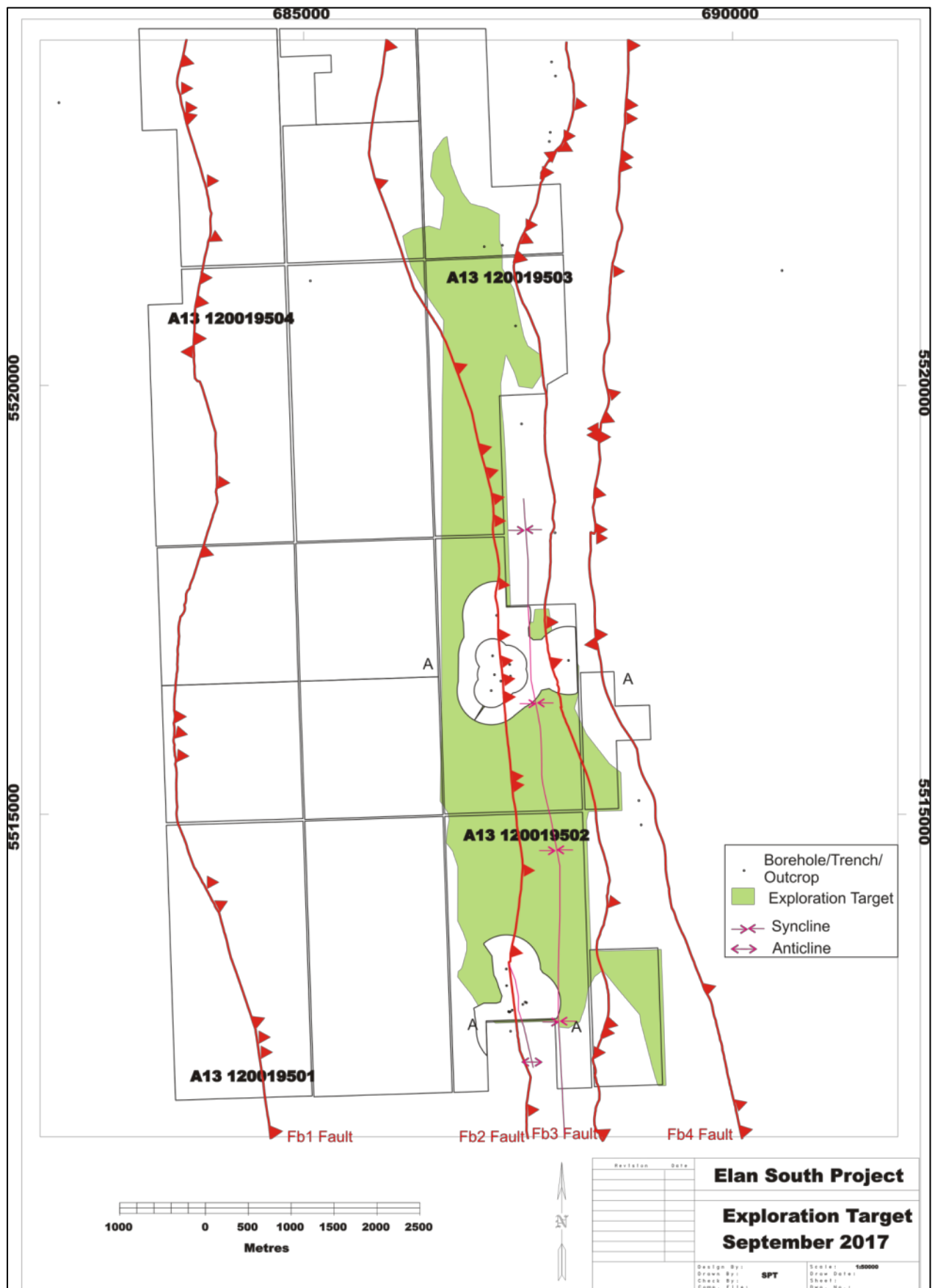
Figure 10 – Exploration Target Area – Elan South – As at 30th September 2017
