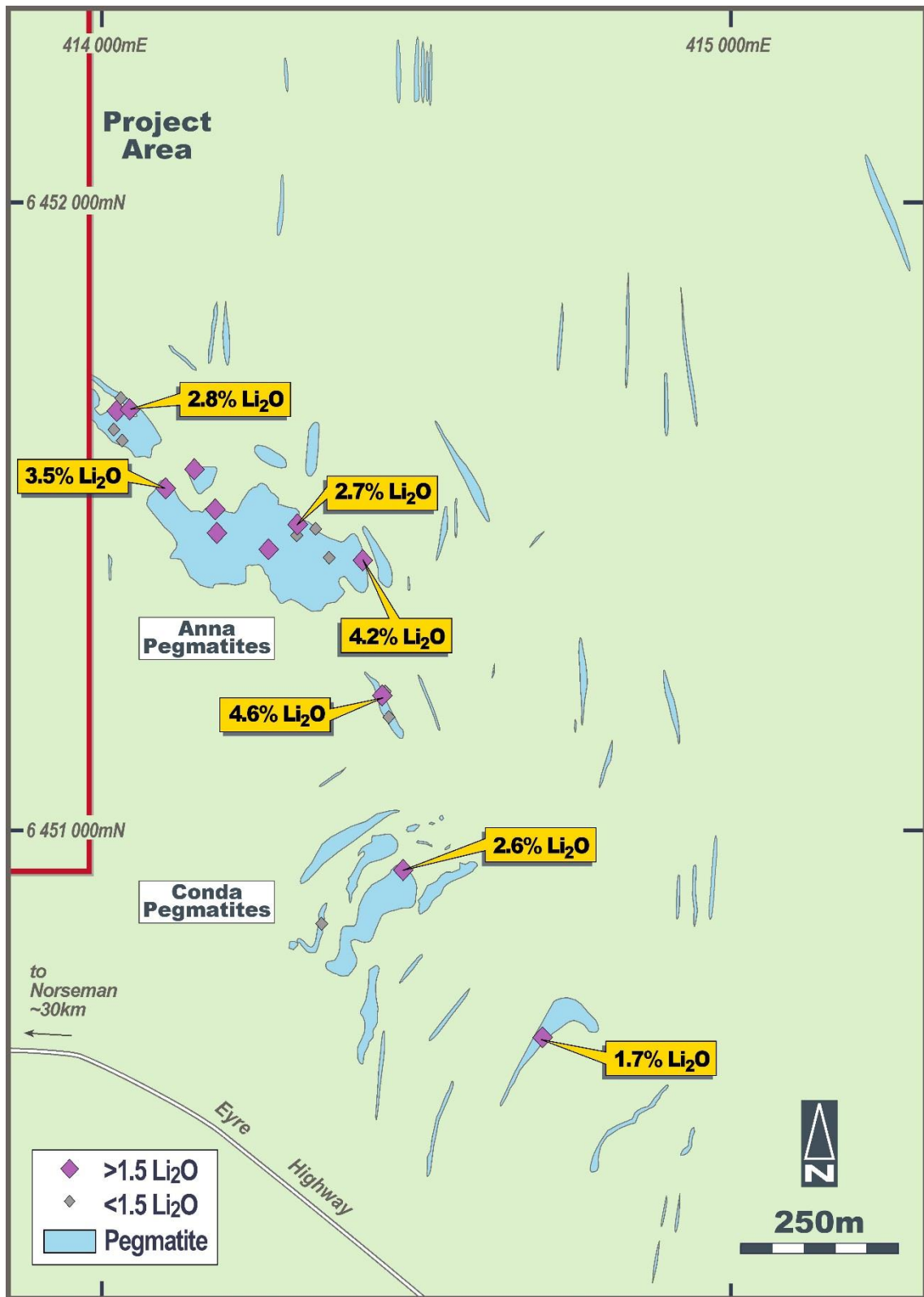
Figure 1: Buldania Project – Geological plan showing mapped pegmatites and Liantown rock chip samples
