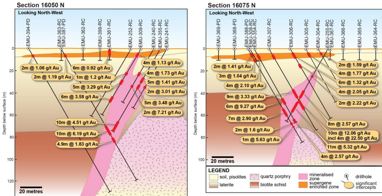
Figure 4. Historical drillhole sections at the southern end of Southwark, along local grid lines 16050 N and 16075 N (see Figure 7 for grid line locations). These sections are adapted from open file report a28505 (Norgold, 1989), showing significant intercepts and interpreted geology.
