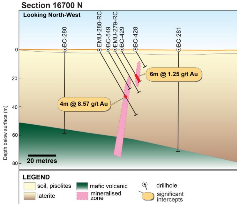
Figure 6. Historical drillhole section at the northern end of Southwark, along local grid line 16700 N (see Figure 7 for grid line location). This section is adapted from information in open file reports a18217 (EZ, 1986) and a28505 (Norgold, 1989), showing significant intercepts and interpreted geology.
