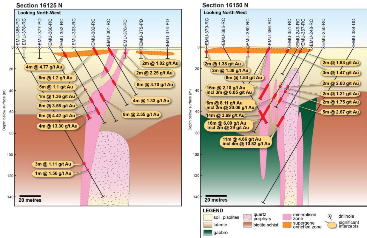
Figure 5. Historical drillhole sections at the southern end of Southwark, along local grid lines 16125 N and 16150 N (see Figure 7 for grid line locations). These sections are adapted from open file report a28505 (Norgold, 1989), showing significant intercepts and interpreted geology.
