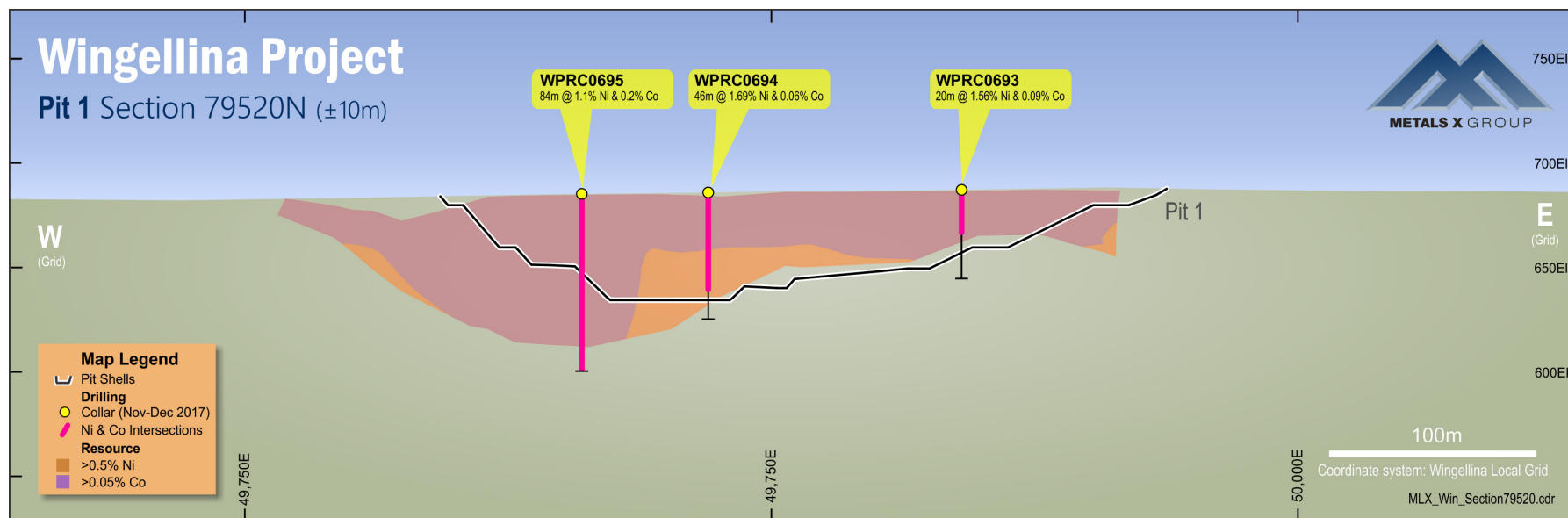
FIGURE 1: CROSS SECTION 79520N – PIT1 SHOWING RECENT DRILL RESULTS (REFER TO FIGURE 3 FOR PIT LOCATION IN PLAN VIEW)
