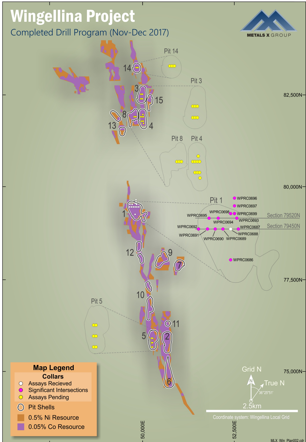
FIGURE 3: COMPLETED WINGELLINA DRILLING PROGRAM SHOWING PIT SHELLS AND DRILL HOLE LOCATIONS
