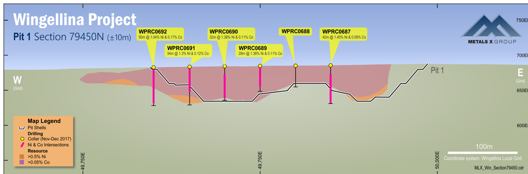
FIGURE 2: CROSS SECTION 79450N – PIT1 SHOWING RECENT DRILL RESULTS (REFER TO FIGURE 3 FOR PIT LOCATION IN PLAN VIEW)
