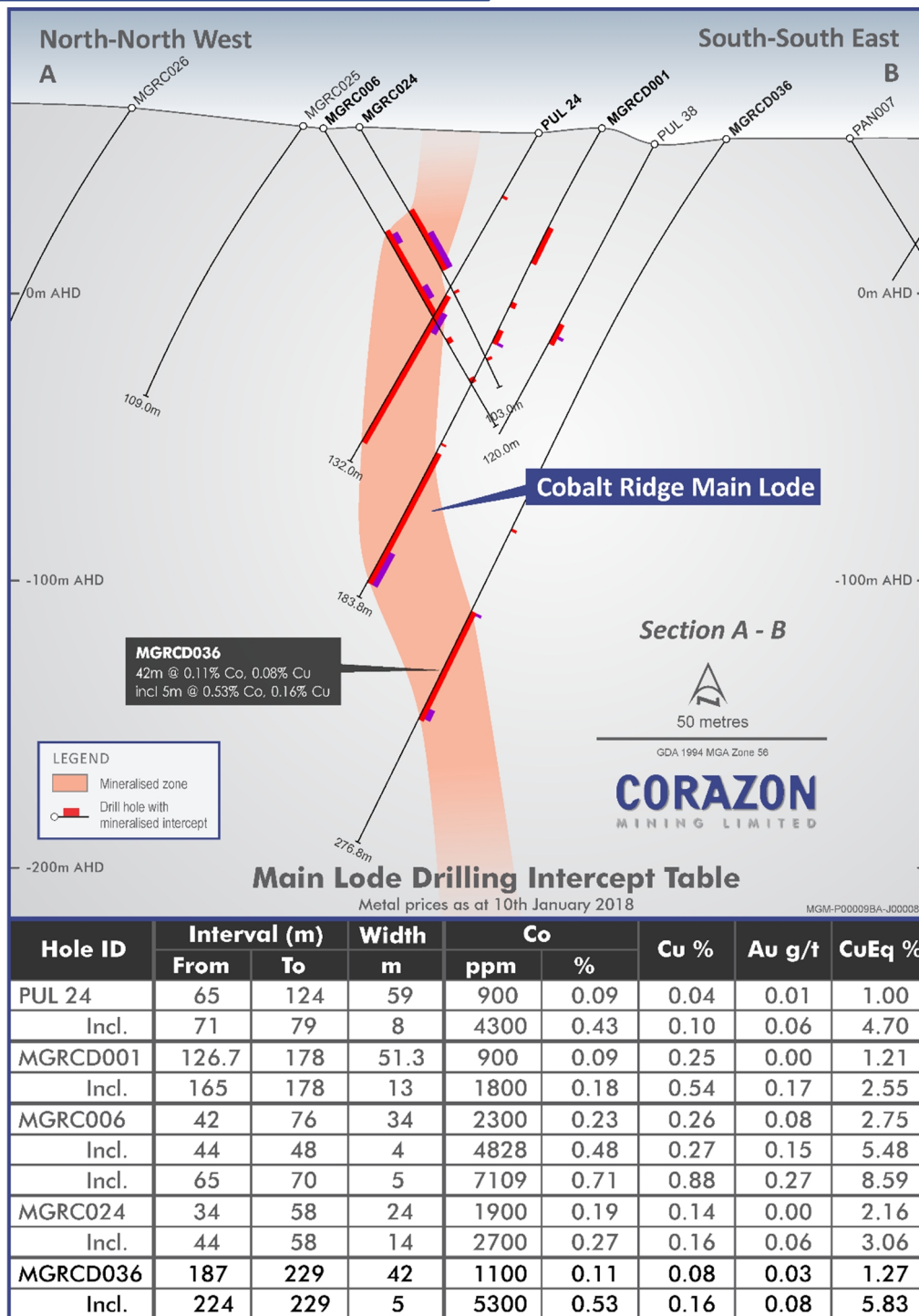
Figure 1: Geological cross-section in line for drill hole MRGC036 (location in Figure 2).
