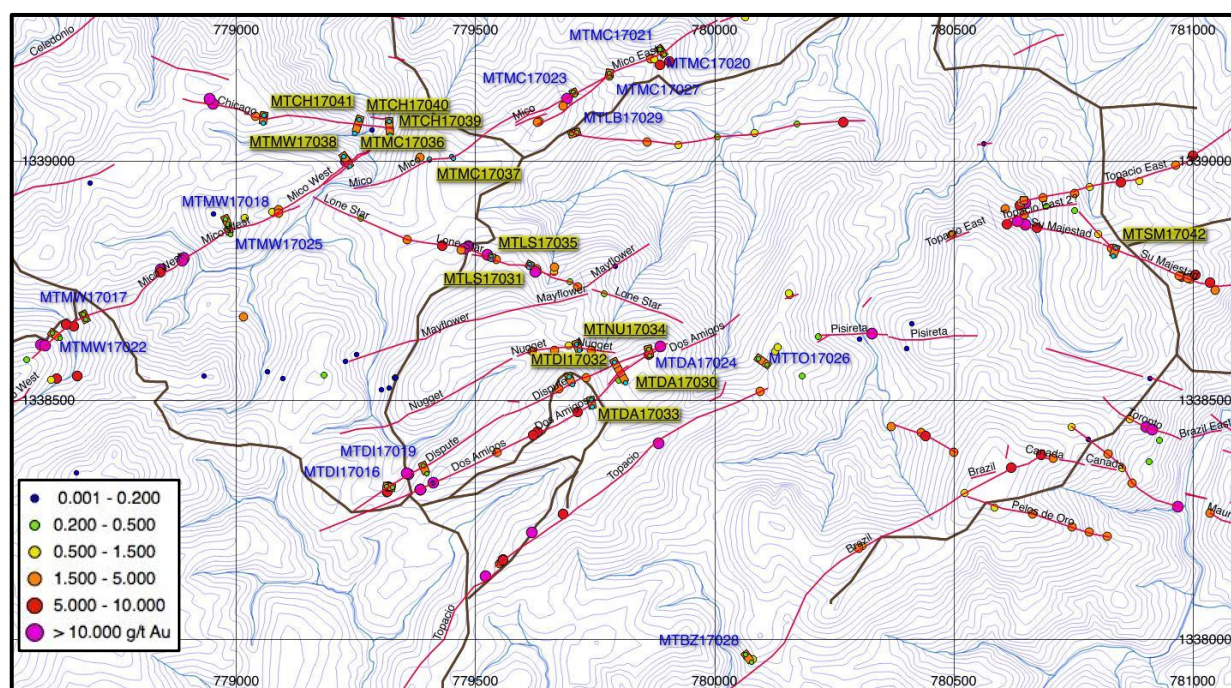
Figure 1 Topacio Phase 3 trenches: Locations (no's 030-042 in yellow) & previous rock chip results
