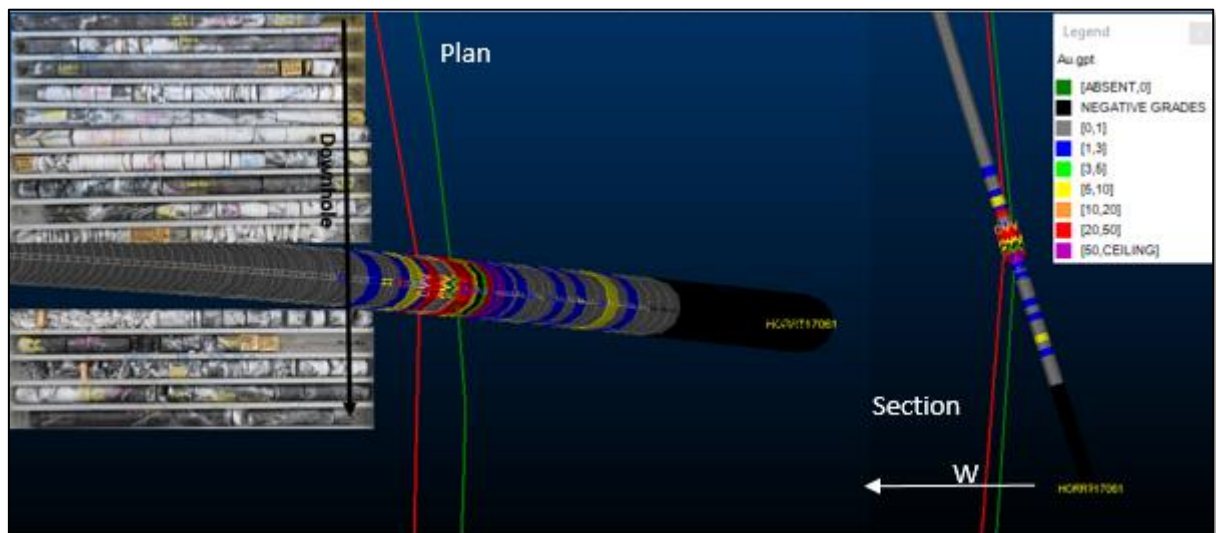
Figure 3. Plan and cross section view of Rubicon K2 with close-up and core photographs of the significant result in hole HORRT17061
