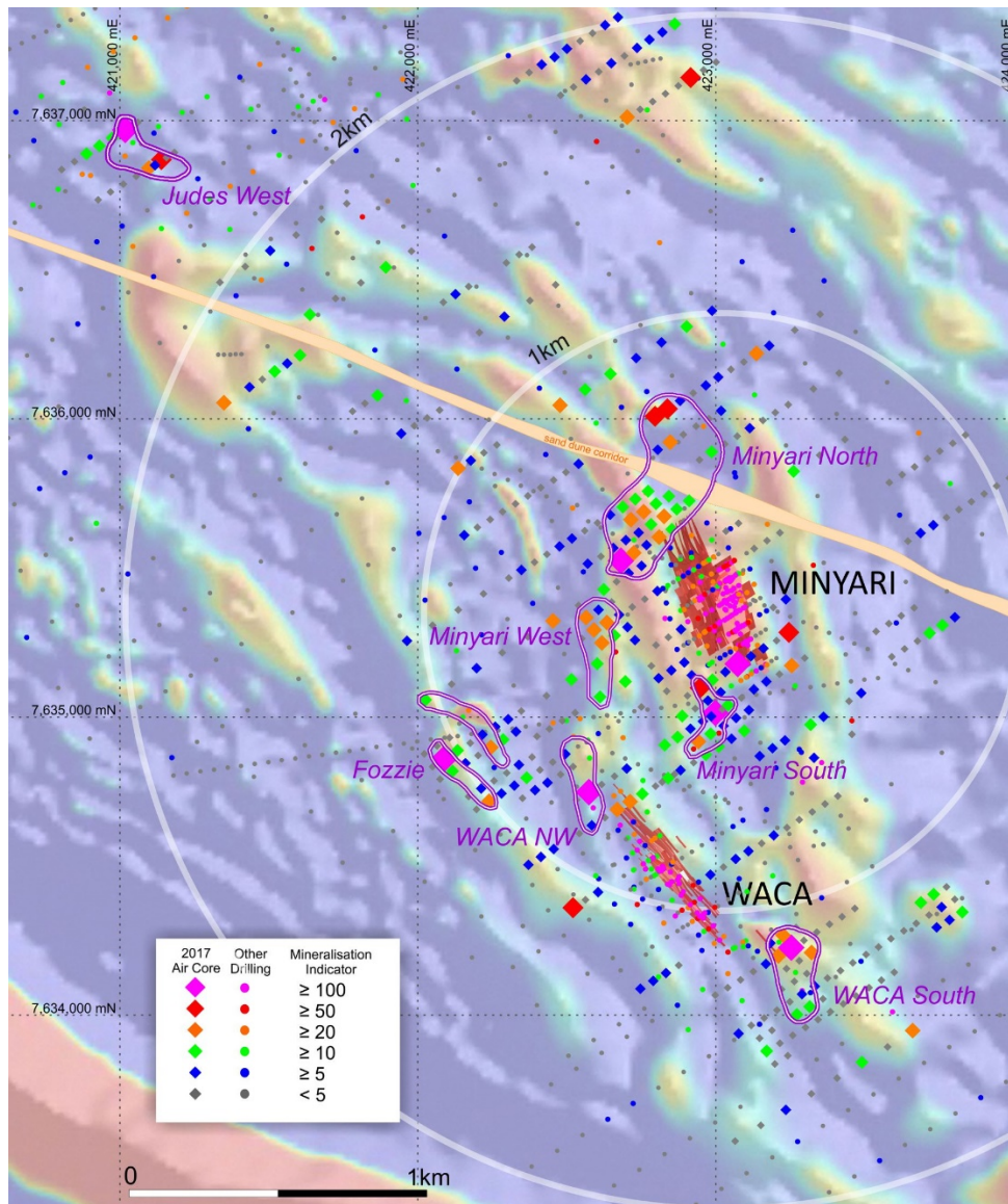
Figure 1: Plan view of the southern region of the Minyari Dome showing prospects, deposits and target locations, and drill holes annotated by “Mineralisation Indicator” (i.e. Au\ ppm \times 100 + Ag\ ppm \times 10 + Bi\ ppm + Cu\ ppm/100 + Co\ ppm/100 + As\ ppm/100 ) maximum value within 60m of surface.
