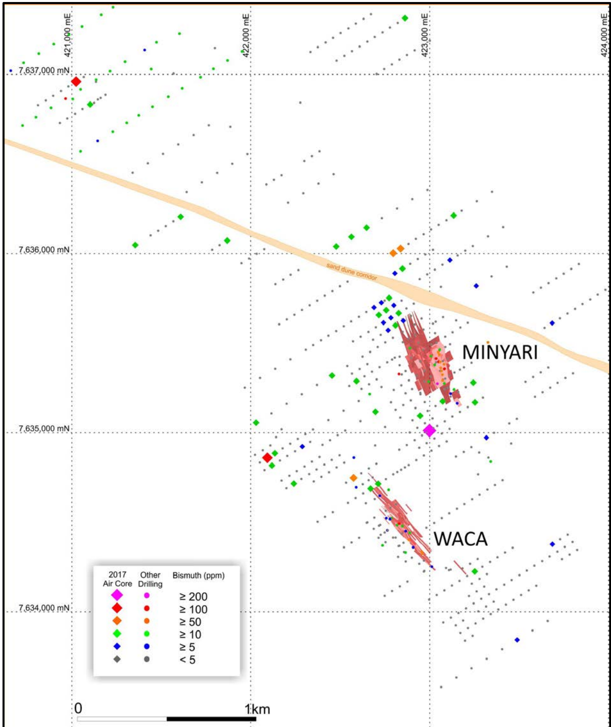
Figure 8: Plan view of the southern region of the Minyari Dome showing deposit locations and drill holes annotated by maximum downhole bismuth value within 60m of surface. Regional GDA94 / MGA Zone 51 co-ordinates, 1km grid.
