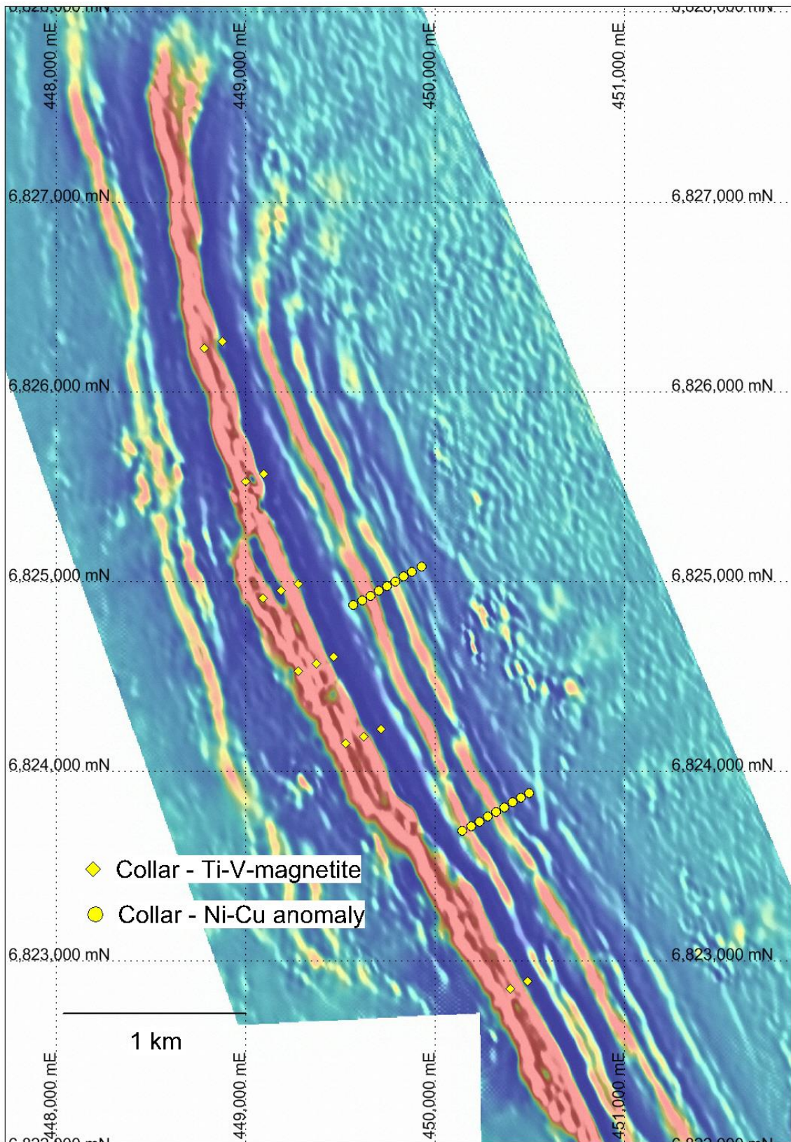
Fig 1. Proposed locations for the 2018 RC drill-holes overlain on the processed magnetic imagery covering the Buddadoo gabbro intrusion and adjacent area. The Ti-V-magnetite collars target a high-order magnetic anomaly and the Ni-Cu collars target second-order magnetic anomalies.
