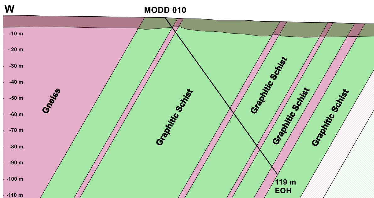
Figure 2. Cross section of MODD010
