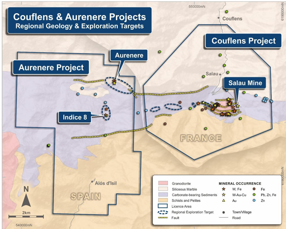
Figure 3: Regional Geology of Couflens and Aurenere Projects
