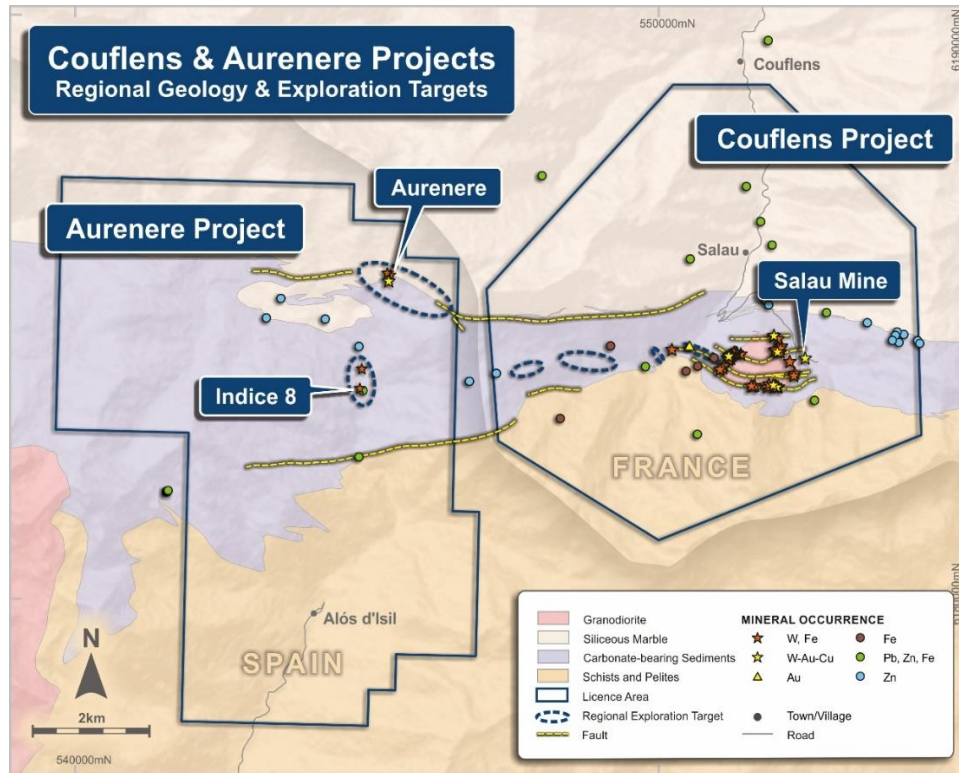
Regional Geology of Couflens and Aurenere Projects
