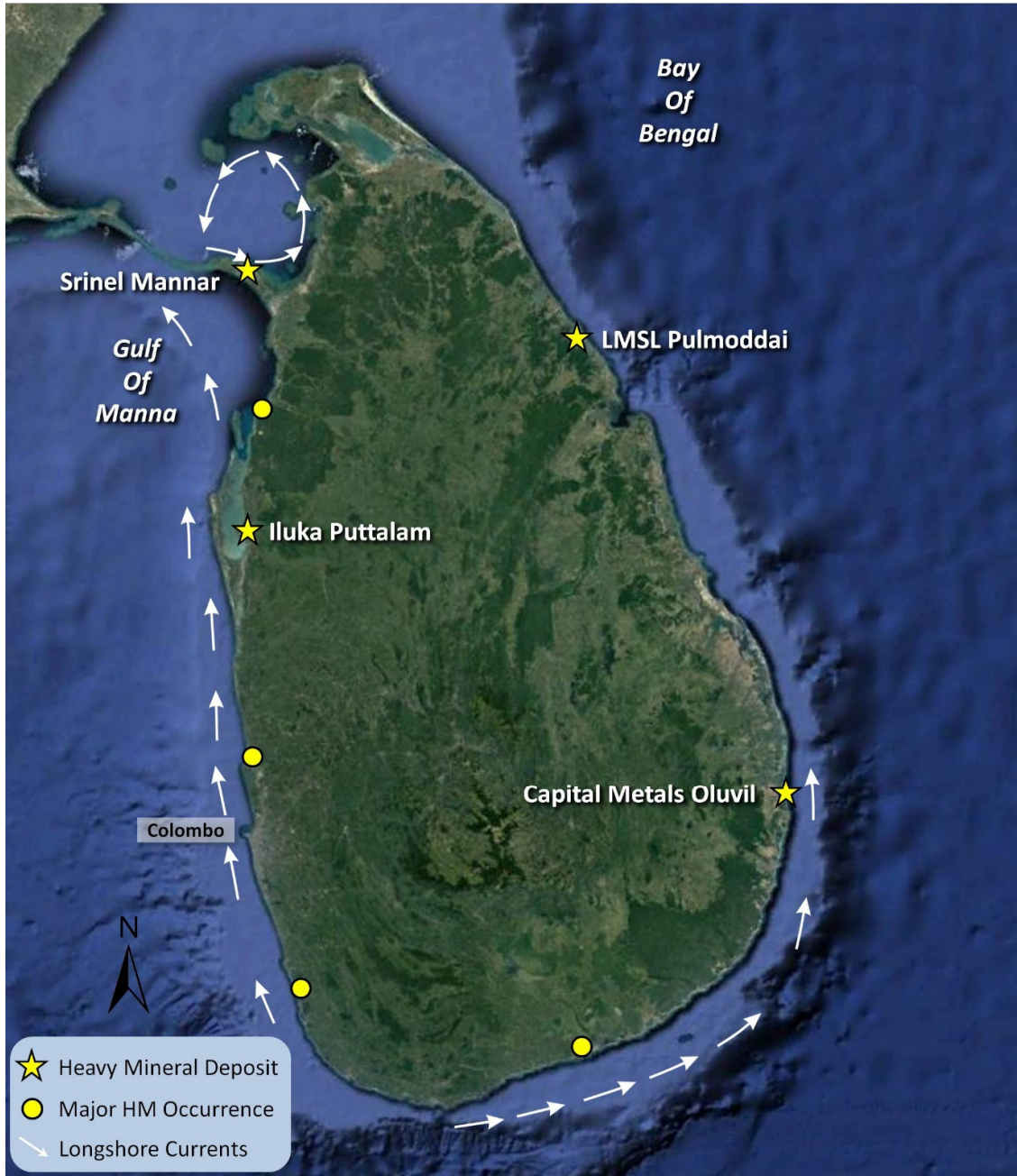
Figure 4 Sri Lankan Heavy Mineral Deposits and Occurrences
