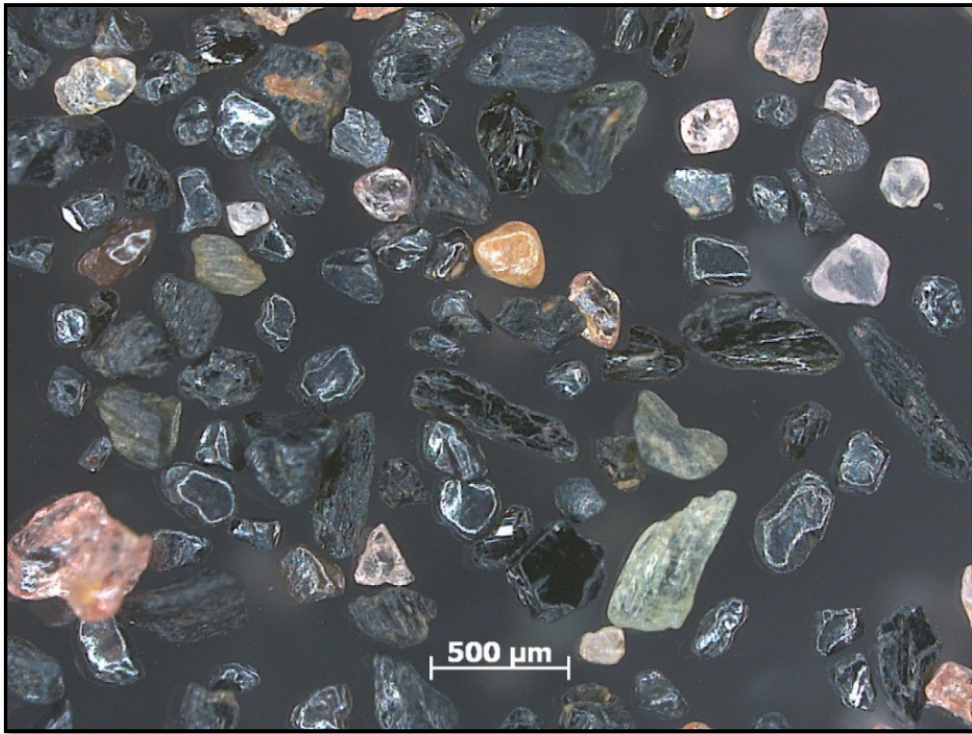
Figure 13 Stereomicroscopic image of magnetic-others fraction
