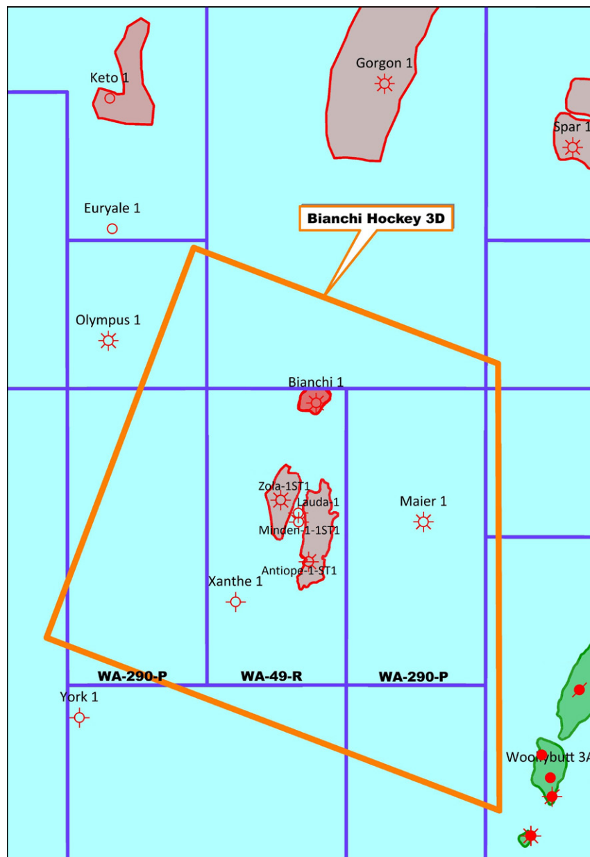
Figure 3 - Bianchi 3D seismic survey
