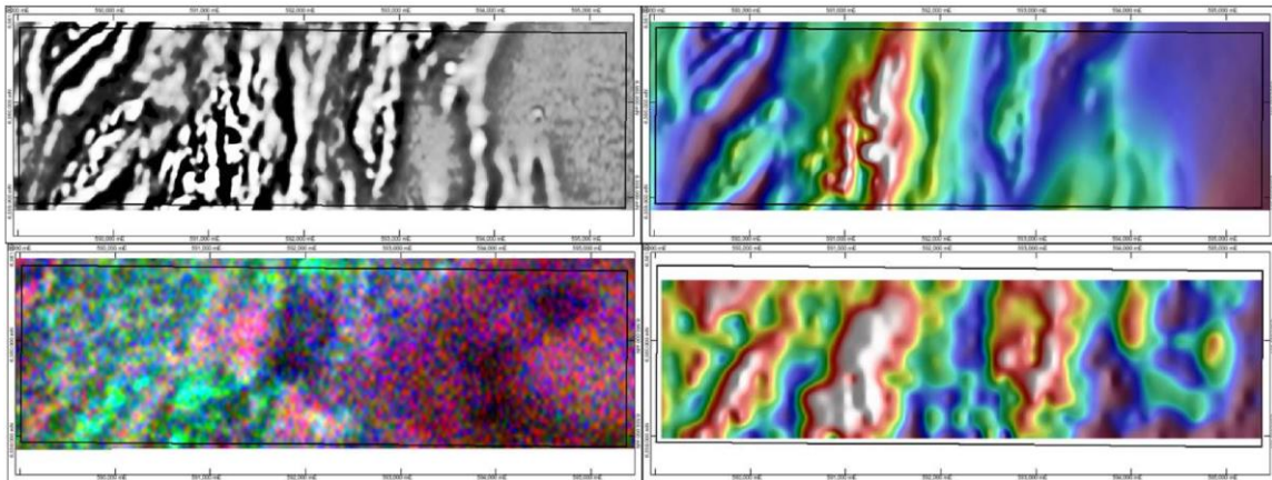
Figure 1: Data collected over the Eastern Block tenements. Clockwise from top left: 2VD Magnetics, RTP magnetics, gravity 1VD (BA267) and ternary radiometrics.
