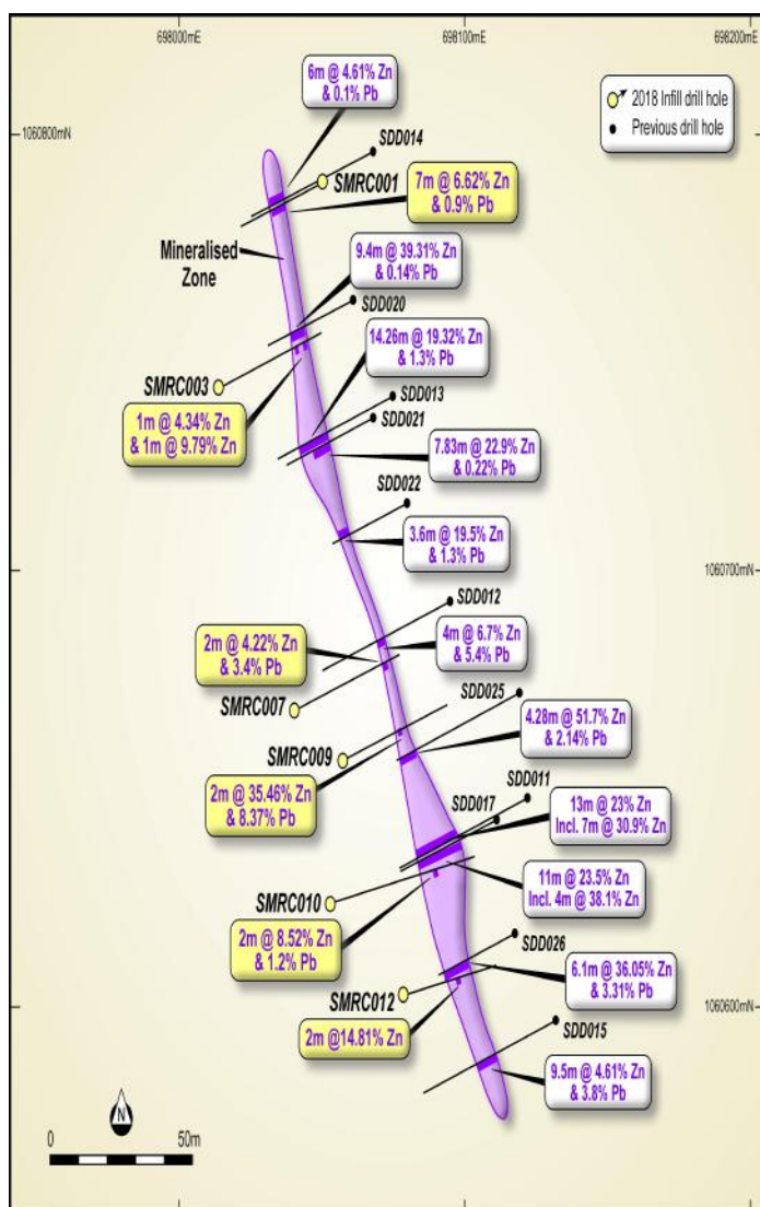
Figure 2: Macy Zinc Drill Hole Locations and Intersection
