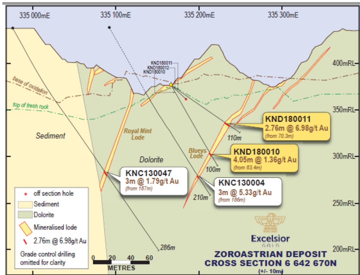
Figure 1: Cross section through 6 642 670N highlighting the most recent drilling into Blueys lode
