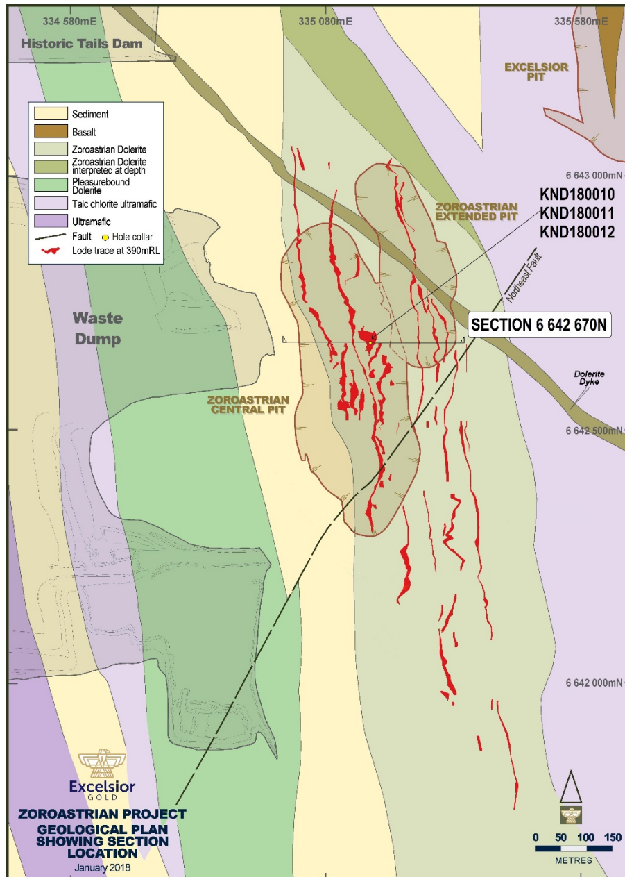
Figure 2: Plan highlighting the collar positions of most recent drilling into Blueys lode
