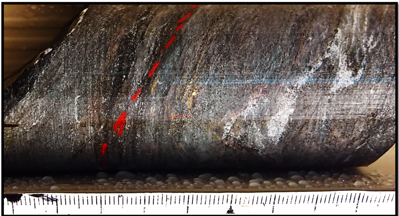
Photo 1: TAN18-DD189: Visible gold at 680.5m – 240 g/t Au
