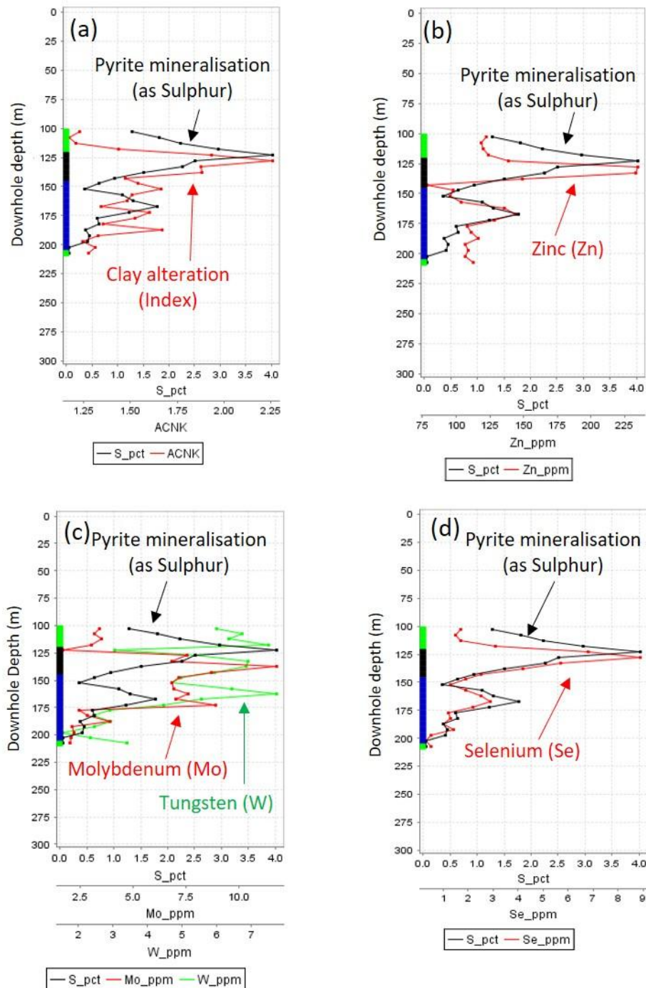
Figure 2 -- Downhole comparison within drillhole RWMEM1-3 of pyrite mineralisation (as wt%S) with (a) clay alteration/destruction of feldspars (as ACNK Index = \text{Al}_2\text{O}_3/\text{CaO} + \text{Na}_2\text{O} + \text{K}_2\text{O} all wt%), (b) Zn concentration (ppm), (c) Mo and W concentrations (ppm), (d) Se concentration (ppm). Showing data from drillhole RWMEM1_3 only (see JORC Table 1 for location) as an example; the same geochemical relationships were found in all drill holes. All geochemistry represents 5m composites of 1m RC drill samples (see JORC Table 1 attached for all procedures). Note that the first 100m of the drill hole was not analysed due to the effect of weathering.
