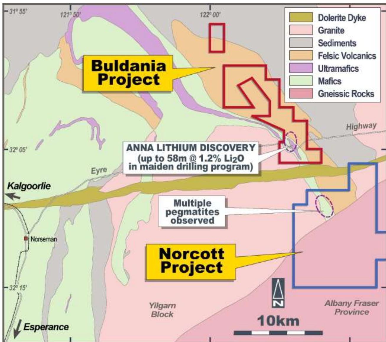
Figure 2: Norcott Lithium Project – Regional geology
