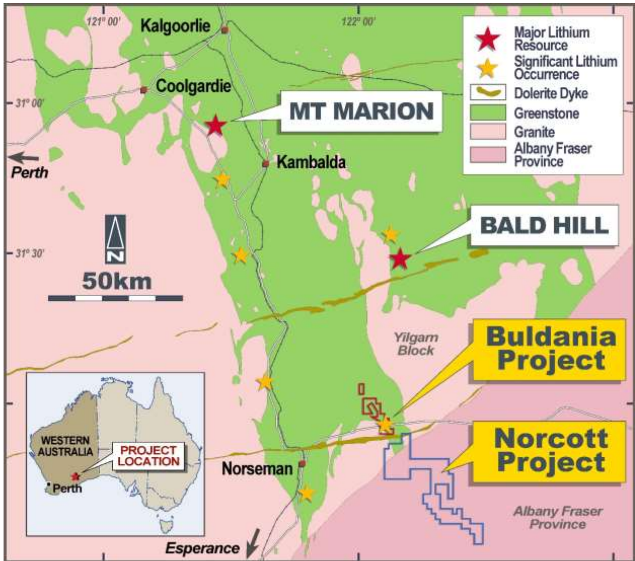
Figure 1: Norcott Lithium Project – Location plan
