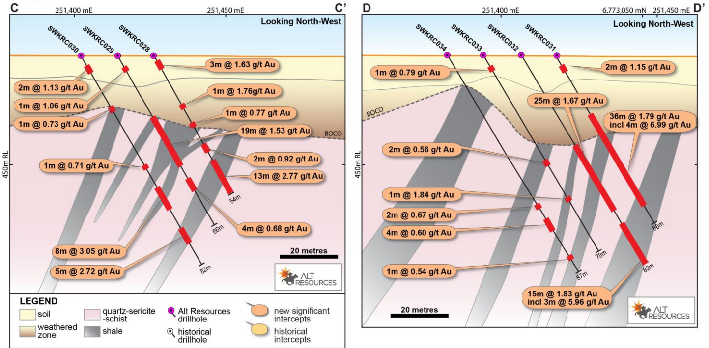
Figure 4. Cross-sections C-C' and D-D' for the new RC drilling at Southwark, Bottle Creek. The location of sections is shown in the plan map in Figure 6. Alt's new drilling results from this announcement are labelled in orange, whilst historical intercepts from previous explorers are labelled in yellow (See open file report a28505).
