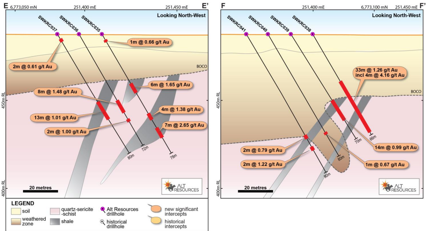
Figure 5. Cross-sections E-E' and F-F' for the new RC drilling at Southwark, Bottle Creek. The location of sections is shown in the plan map in Figure 6.
