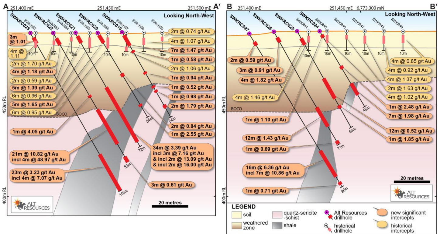
Figure 3. Cross-sections A-A' and B-B' for the new RC drilling at Southwark, Bottle Creek. The location of sections is shown in the plan map in Figure 6. Alt's new drilling results from this announcement are labelled in orange, whilst historical intercepts from previous explorers are labelled in yellow (See open file report a28505).
