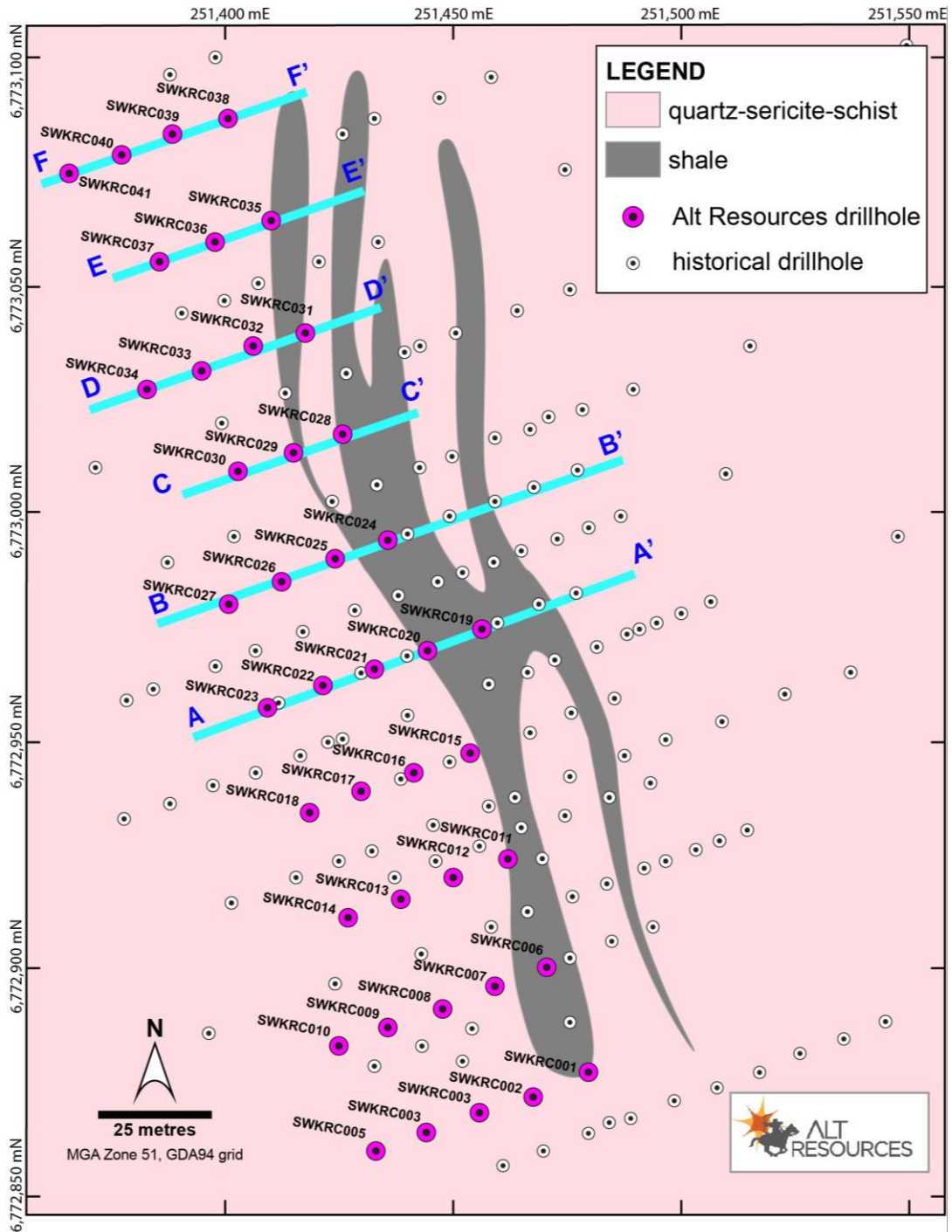
Figure 6. Plan map of new drilling at the Southwark Deposit, Bottle Creek, with sections labelled as shown in this announcement (Figure 3-5).
