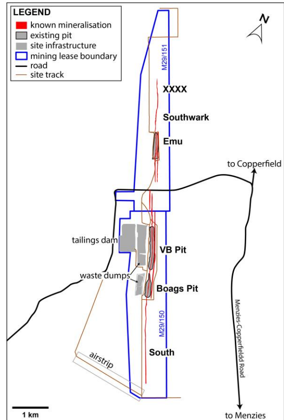
Figure 9. Site layout at Bottle Creek, showing historical VB and Boags open pits as well as the location of un-mined mineralisation at Emu, Southwark and XXXX.
